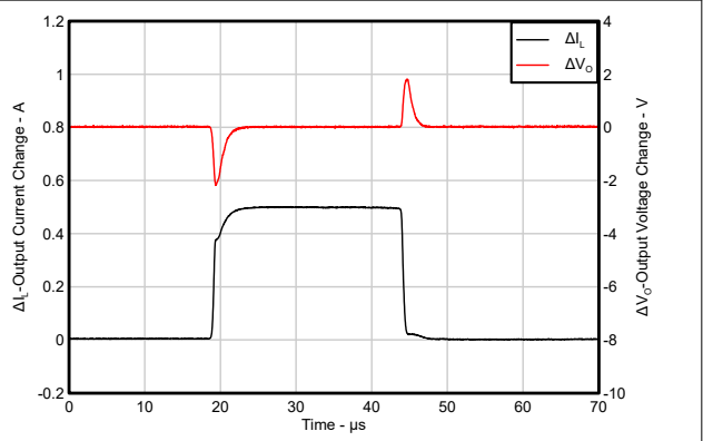
V_{IN} = 15V , V_{OUT} = 1.25V , I_L = 10mA \text{ to } 500mA , C_{ADJ} = 0\mu F , C_{OUT} = 0\mu F
