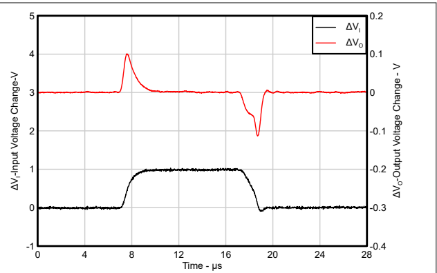
V_{IN} = 14.5V \text{ to } 15.5V , V_{OUT} = 1.25V , I_L = 50mA , C_{ADJ} = 0\mu F , C_{OUT} = 0\mu F
