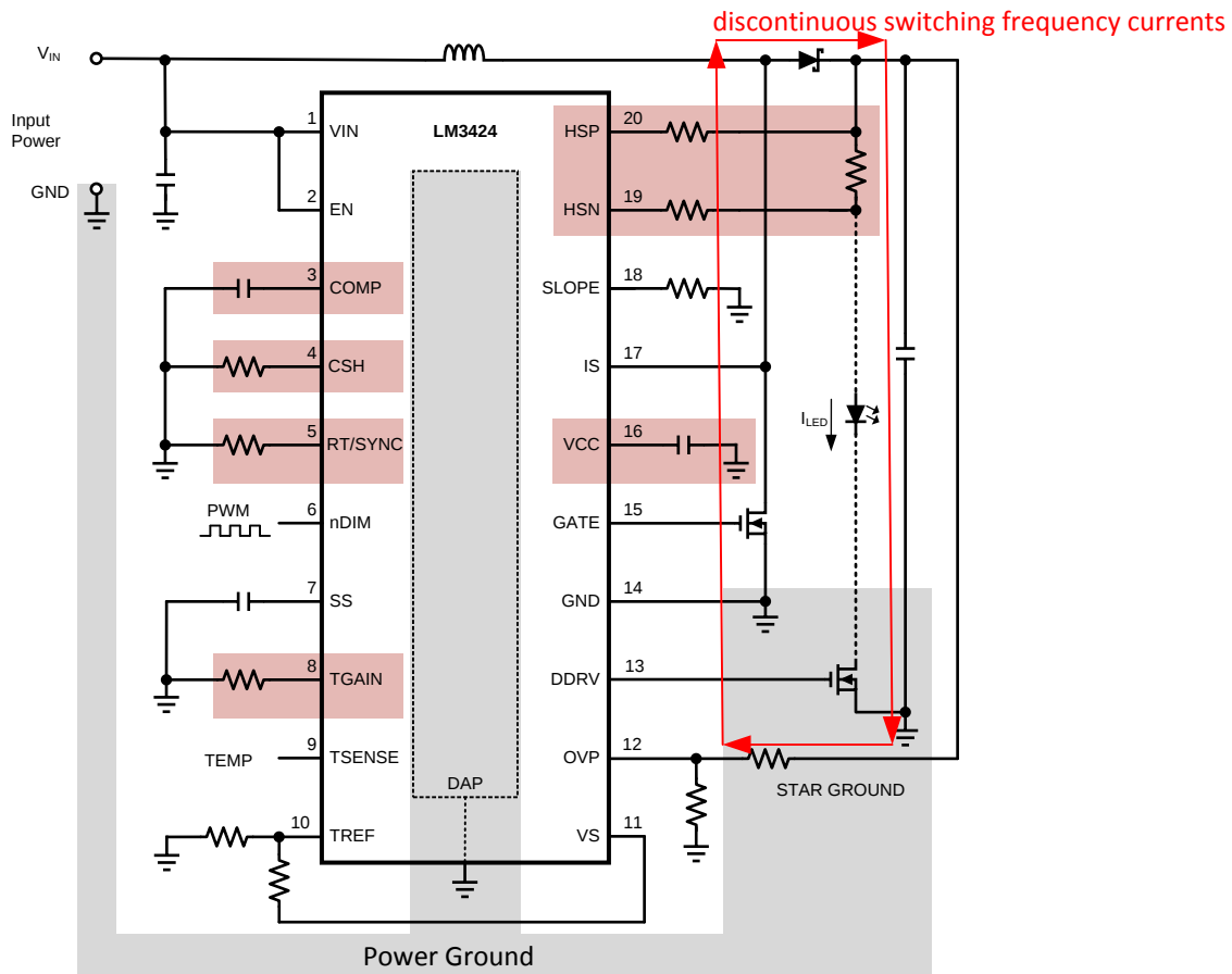
Figure 48. Layout Recommendation
