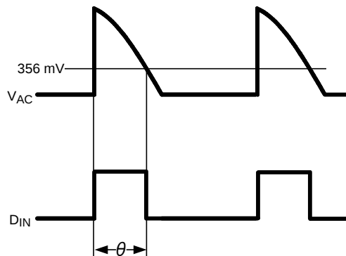
Figure 27. Phase Angle Demodulation
