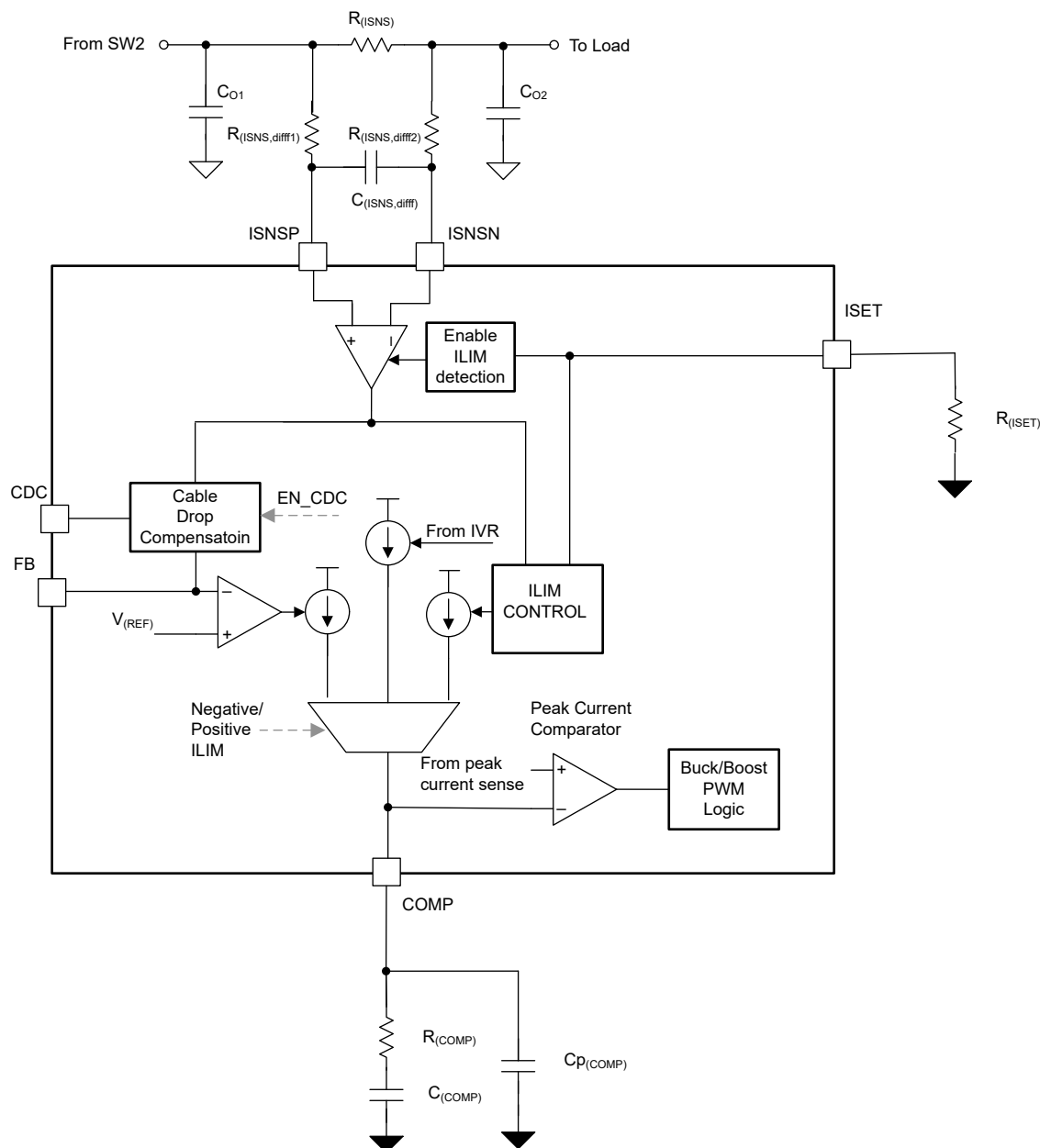
Figure 8-17. Current Monitor Functional Block Diagram
