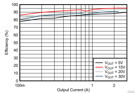
Efficiency vs Output Current, V_{IN} = 12V , PSM
