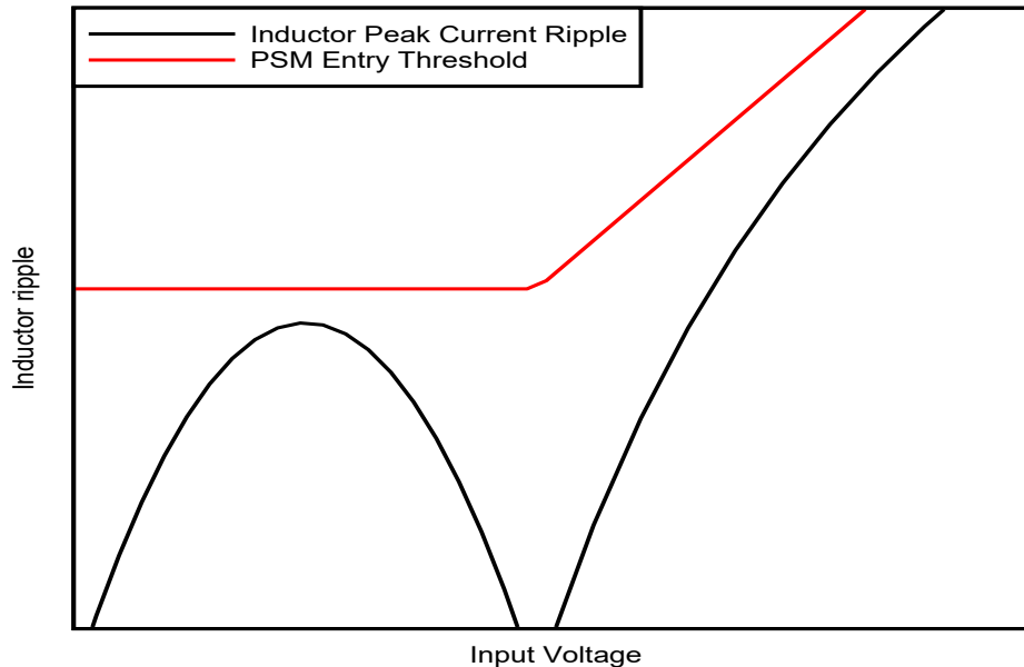
Figure 8-7. Generic Graph of PSM Entry Threshold And Ripple Current Versus Input Voltage
