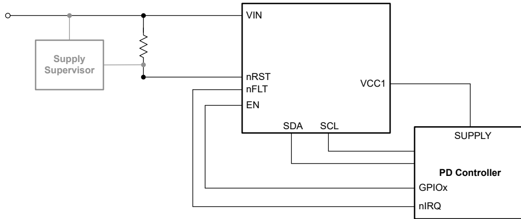
Figure 8-11. Simplified Schematic
