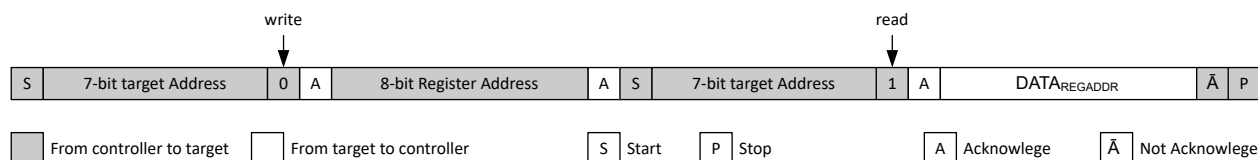
Figure 8-34. Single READ From a Defined Register Address
