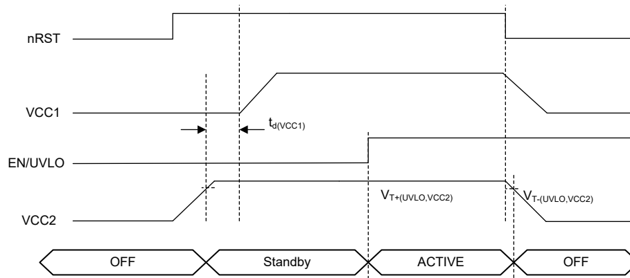
Figure 8-12. Timing Diagram VCC Regulator
