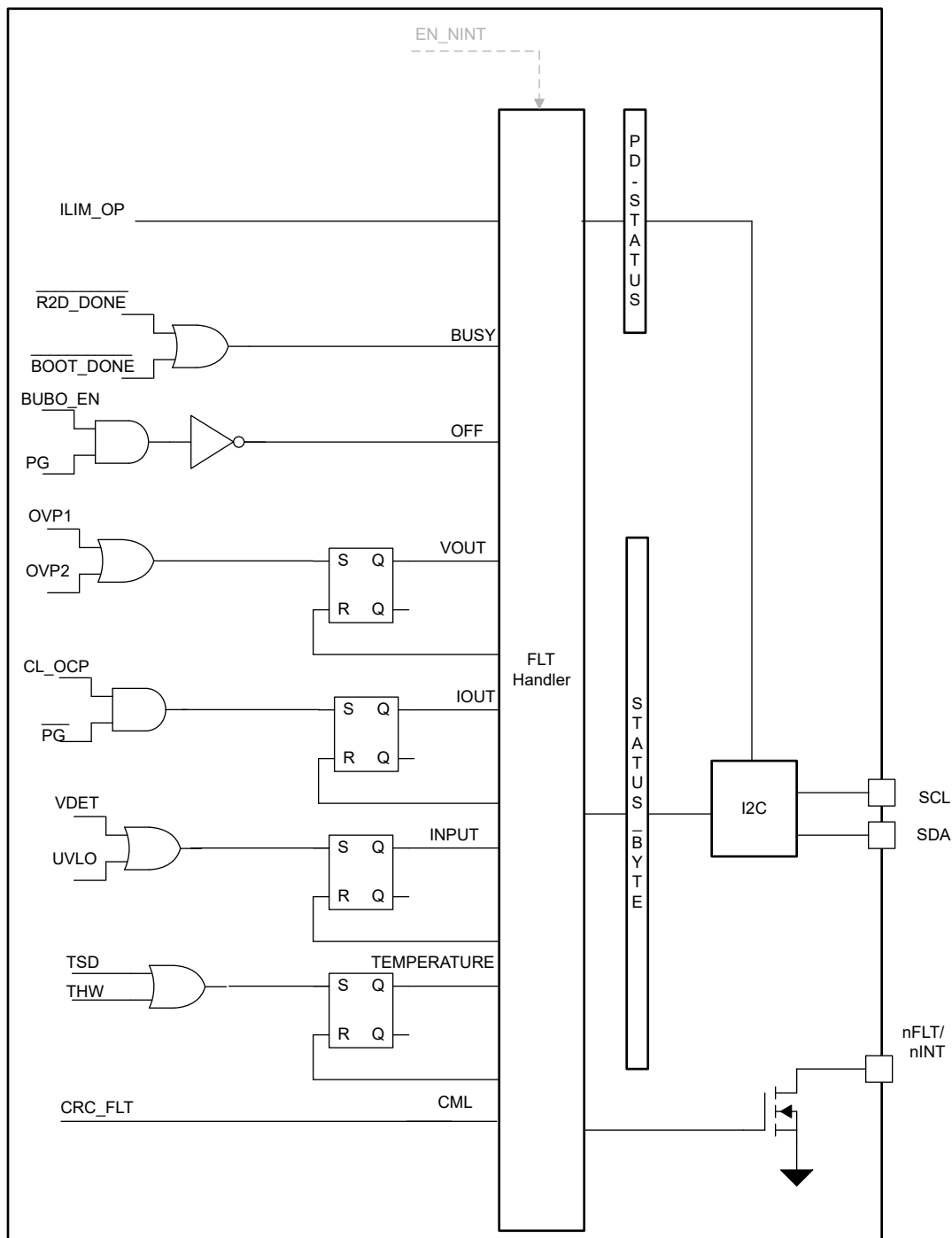
Figure 8-27. Functional Block Diagram Fault Handler
