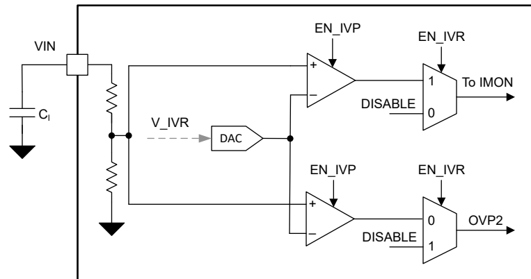
Figure 8-29. Functional Block Diagram IVP/IVR
