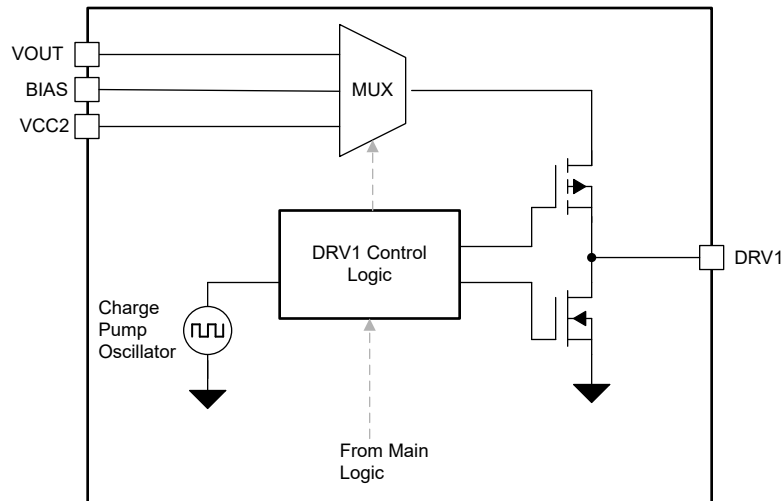
Figure 8-23. Functional Block Diagram - DRV Pin
