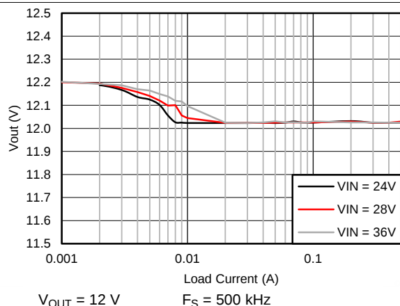
Figure 85. Output Voltage Regulation
