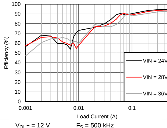
Figure 84. Efficiency
