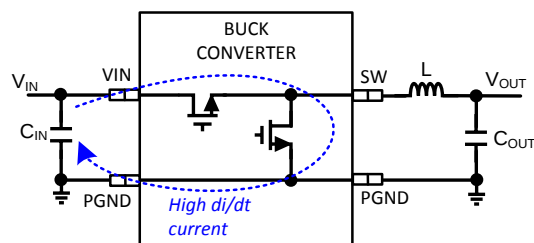
Figure 106. Buck Converter High di / dt Path
