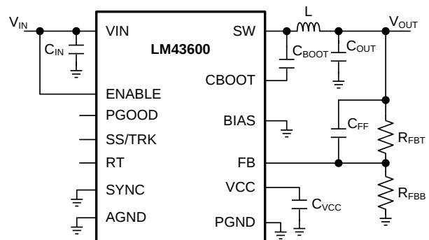
Figure 45. LM43600 Basic Schematic for V_{OUT} < 3.3 V, Tie BIAS to Ground
