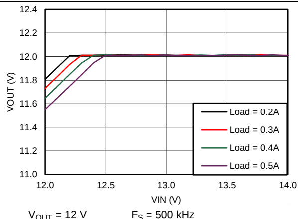
Figure 86. Dropout Curve
