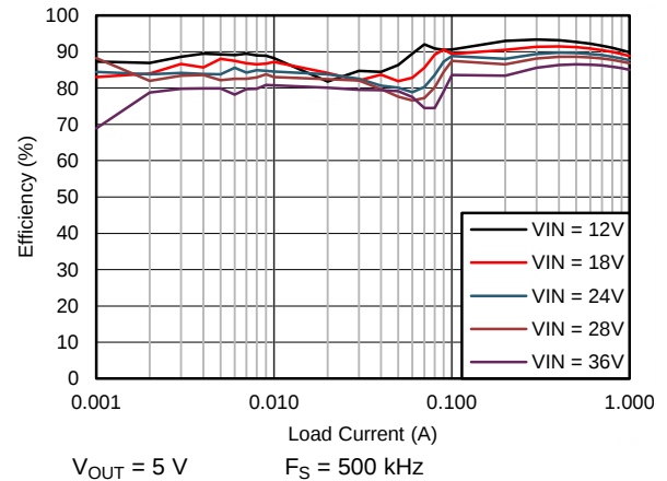
Figure 60. Efficiency
