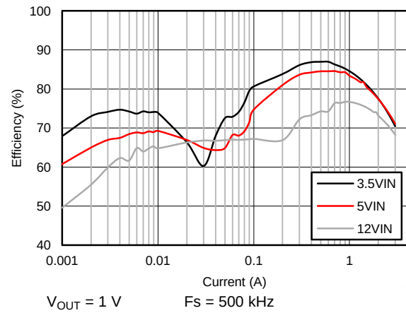
Figure 50. Efficiency
