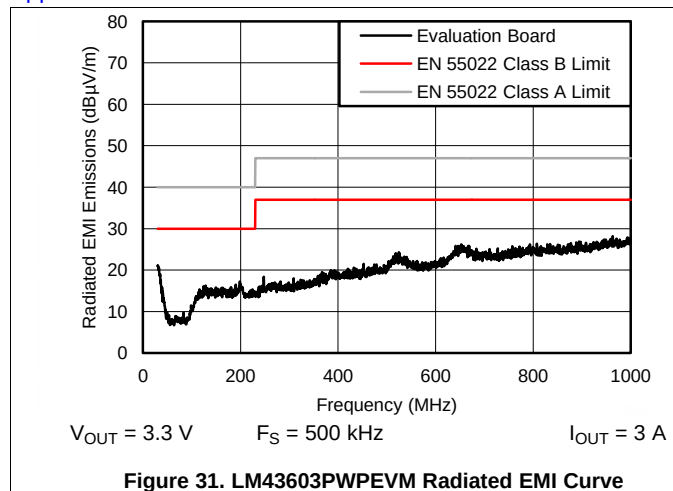
Figure 31. LM43603PWPEVM Radiated EMI Curve
