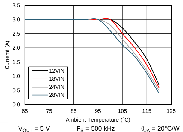
Figure 78. Derating Curve
