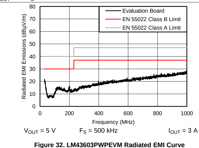
Figure 32. LM43603PWPEVM Radiated EMI Curve
