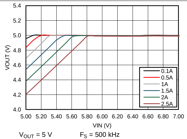
Figure 76. Drop-out Curve
