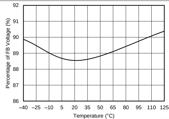
Figure 29. PGOOD UVP Falling Threshold vs Junction Temperature
