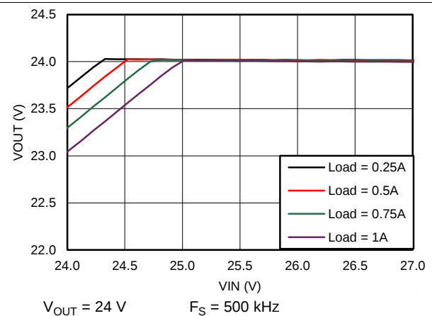
Figure 80. Dropout Curve
