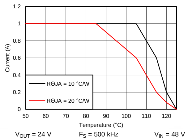
Figure 82. Derating Curve
