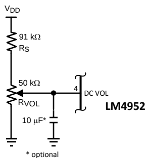
Figure 44. Typical Circuit Used for DC Voltage Volume Control
