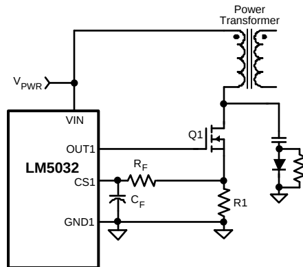
Figure 26. Current Sense Using a Source Sense Resistor (R1)
