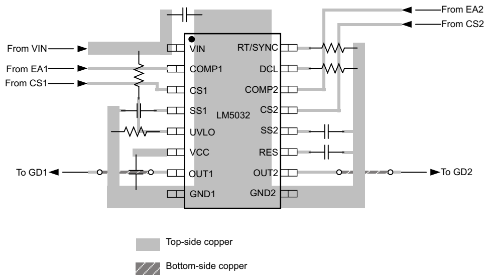
Figure 33. Layout Example
