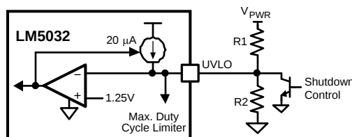
Figure 23. Shutdown Control
