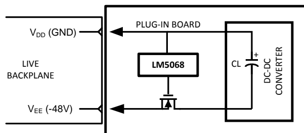
Figure 23. LM5068 Topology
