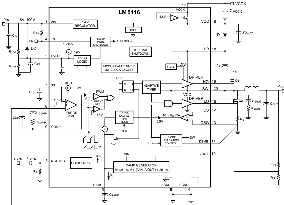
Figure 2. Typical Application
