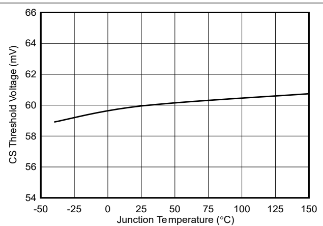
Figure 6-22. Current Sense Threshold vs Temperature
