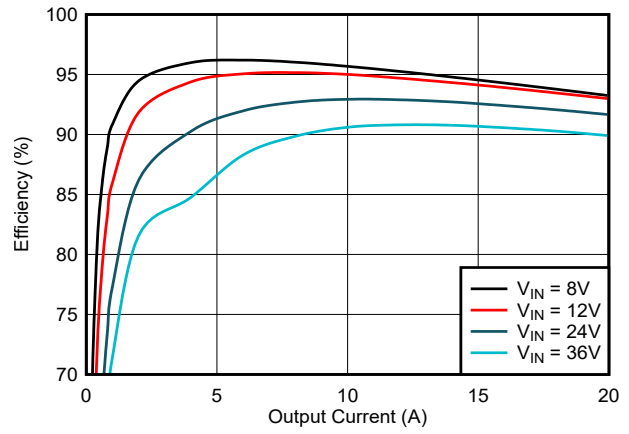
Figure 6-2. Efficiency vs Load, 3.3V Output
