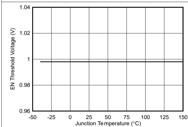
Figure 6-23. EN Rising Threshold Voltage vs Temperature
