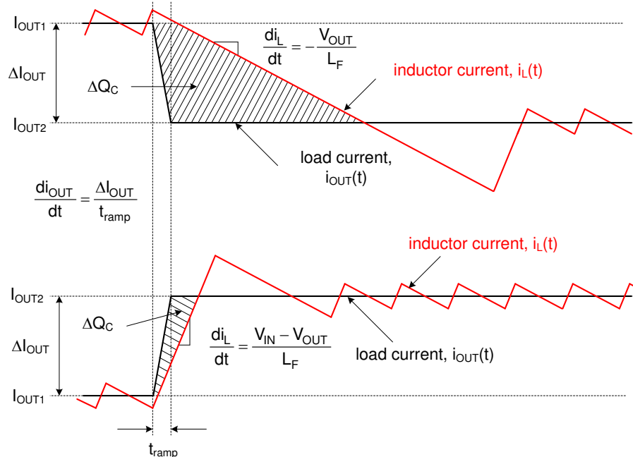
Figure 8-1. Load Transient Response Representation Showing C_{OUT} Charge Surplus or Deficit
