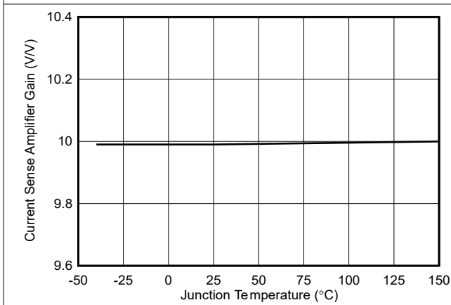
Figure 6-21. Current Sense Amplifier Gain vs Temperature
