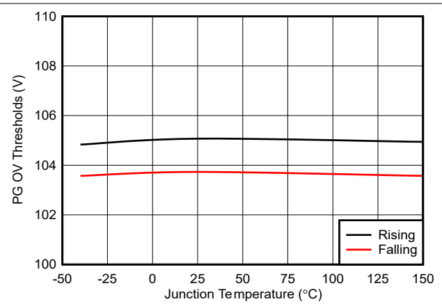
Figure 6-20. PG OV Thresholds vs Temperature
