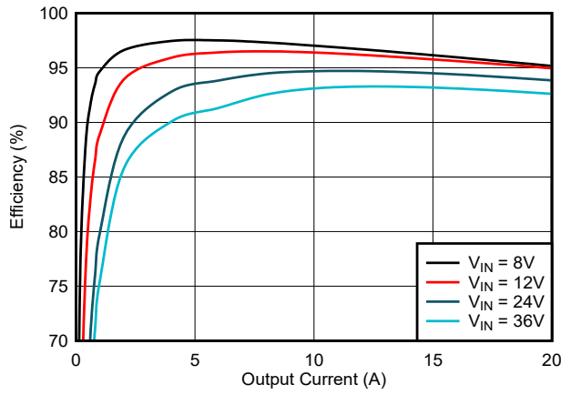
Figure 6-1. Efficiency vs Load, 5V Output
