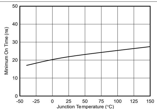
Figure 6-24. Minimum On Time vs Temperature
