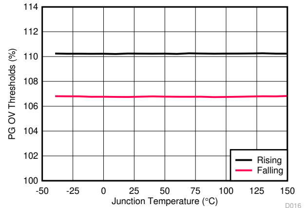
Figure 8-14. PG OV Thresholds Versus Temperature
