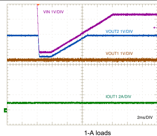
Figure 10-10. Cold-Crank Response to V_{IN} = 3.8\text{ V}
