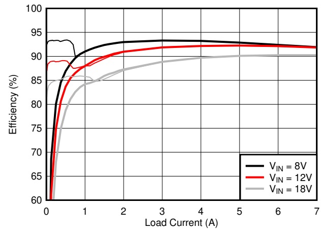
Figure 10-6. Efficiency Versus I_{OUT}
