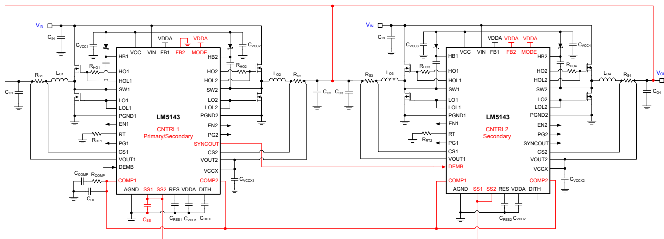
Figure 9-10. Multiphase Regulator Schematic Configured for Single-Output Interleaved Operation
