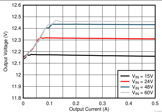
Figure 7-4. Load and Line Regulation Performance
