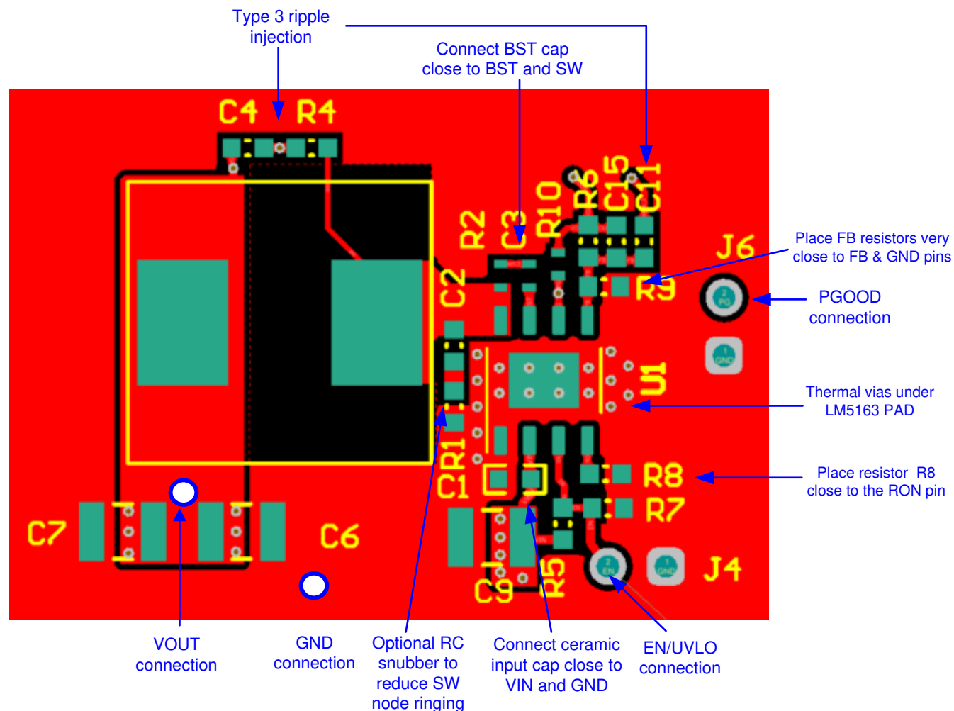
Figure 7-17. LM5163-Q1 Single-Sided PCB Layout Example
