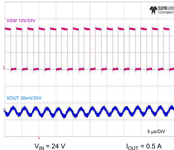
Figure 7-15. Full-Load Switching
