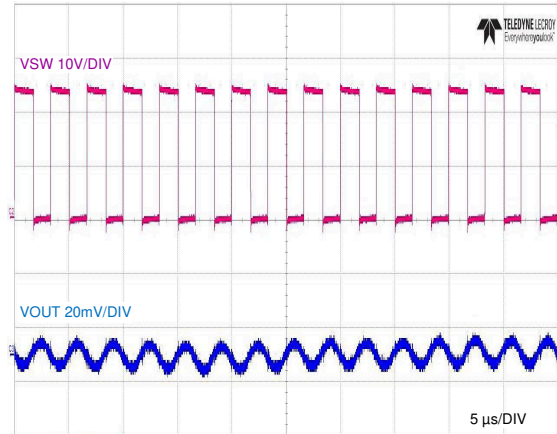
Figure 8-15. Full-Load Switching
