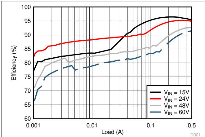
Figure 8-2. Conversion Efficiency (Log Scale)
