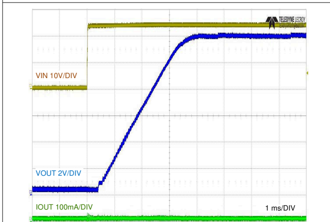
Figure 8-6. No-Load Start-up with VIN
