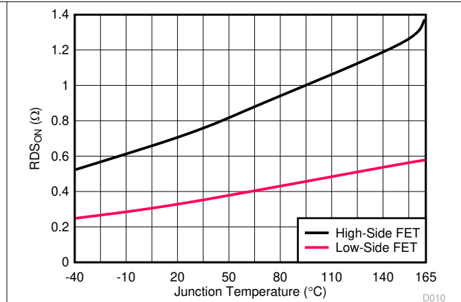
Figure 6-8. MOSFETs On-State Resistance versus Temperature
