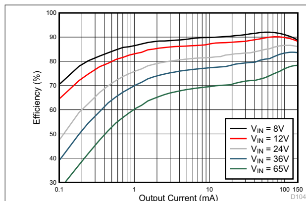
Figure 8-27. Efficiency
