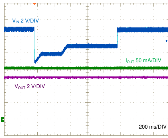
I_{OUT} = 150 mA Figure 8-13. Input Transient (Automotive Cold Crank Profile)
