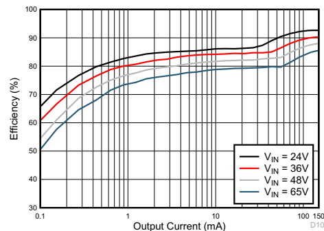
Figure 6-4. Converter Efficiency: 3.3 V, 150 mA, COT
