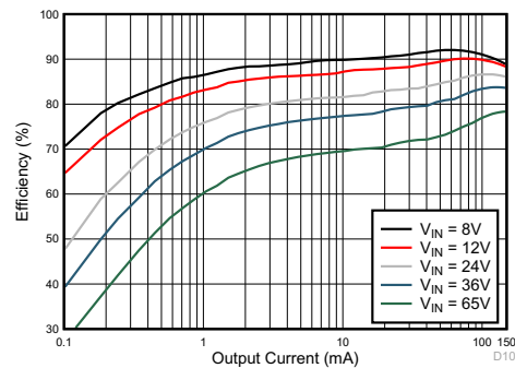
Figure 6-2. Converter Efficiency: 5 V, 150 mA, COT
