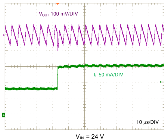
V_{IN} = 24 V Figure 8-12. Load Transient, 50 mA to 150 mA, 1 A/ \mu s
