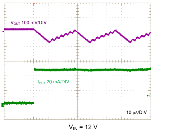
Figure 8-19. Load Transient, 0 mA to 50 mA, 1 A/ \mu\text{s}
