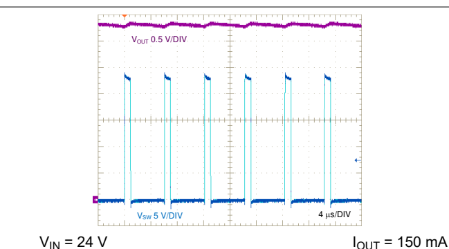
Figure 8-28. SW Node and Output Ripple Voltages, Full Load
