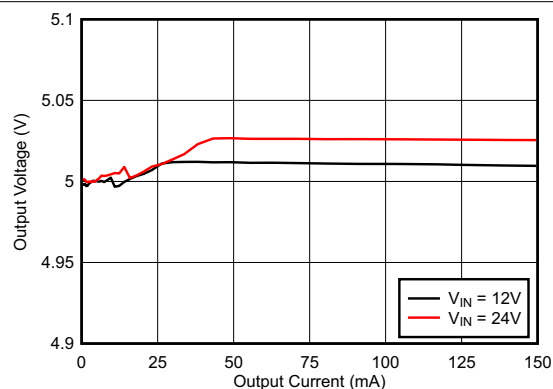
Figure 8-3. Load Regulation
