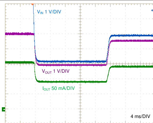
V_{IN} = 24 V 30- \Omega Load Figure 8-9. Enable ON and OFF
