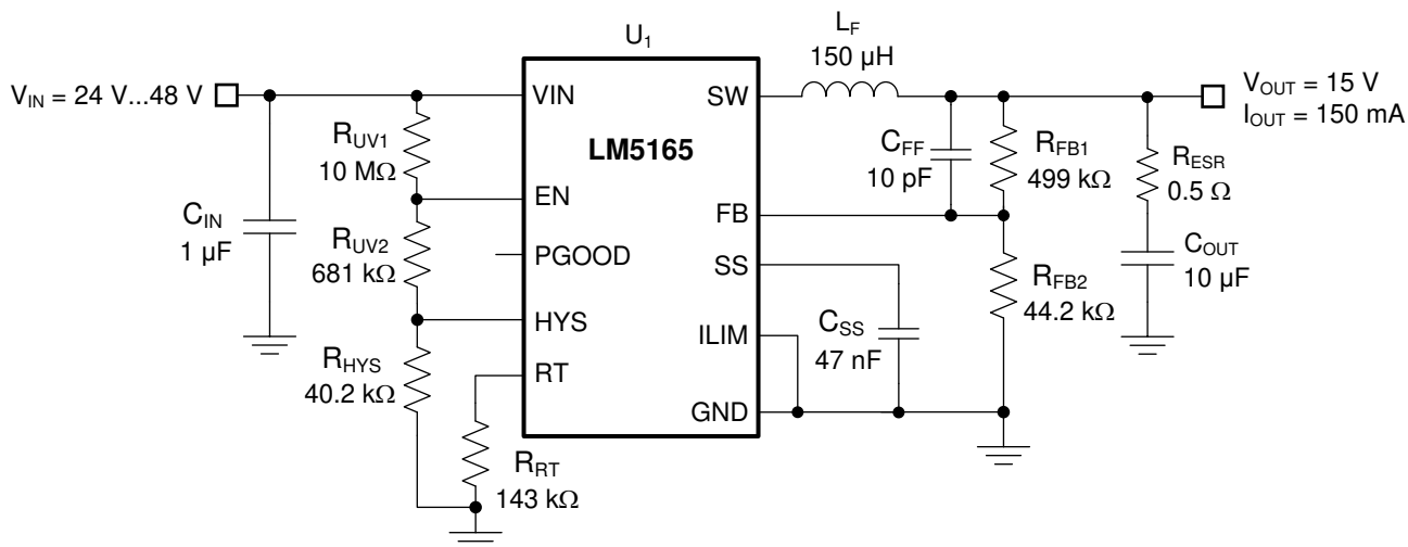
Figure 8-29. Schematic for Design 5 With V_{IN(nom)} = 36 V, V_{OUT} = 15 V, I_{OUT(max)} = 150 mA, F_{SW(nom)} = 600 kHz
