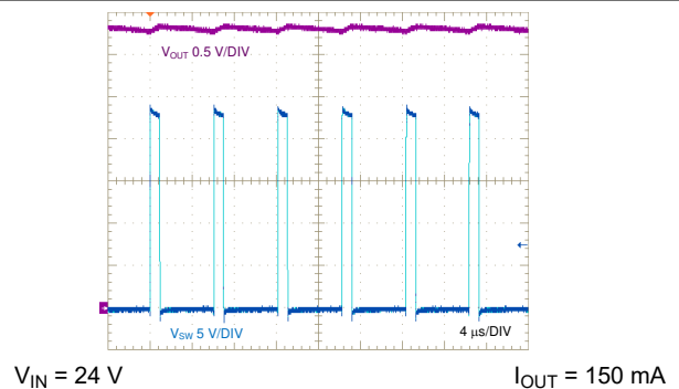
Figure 8-28. SW Node and Output Ripple Voltages, Full Load
