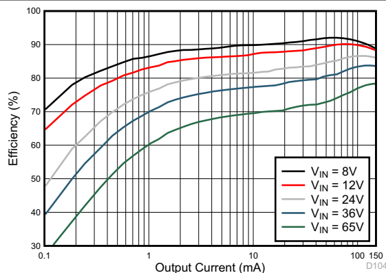
Figure 8-27. Efficiency
