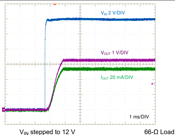
Figure 8-17. Start-Up, Full Load
