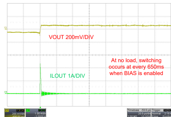
Figure 9-9. No Load Operation in PFM Mode, V_{SUPPLY} = 48V , I_{LOAD} = 0A
