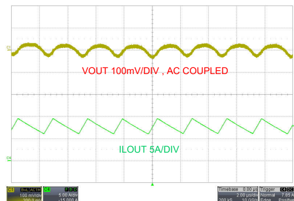
Figure 9-8. Output Ripple, V_{SUPPLY} = 48V , I_{LOAD} = 8A
