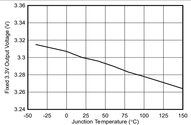
Figure 6-6. Fixed Output Voltage vs Temperature, V_{OUT} = 3.3\text{V}
