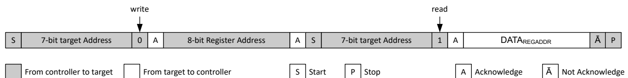
Figure 7-11. Single READ From a Defined Register Address
