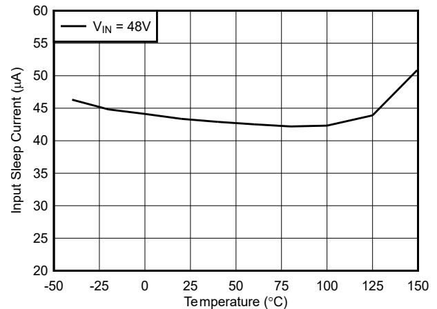
Figure 6-4. Input Sleep Current vs Temperature, V_{OUT} = 5\text{V}
