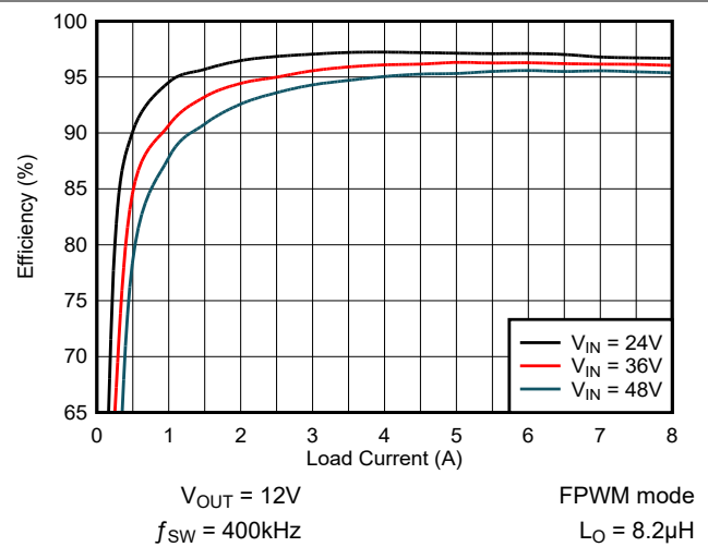
Figure 6-2. Efficiency FPWM Mode
