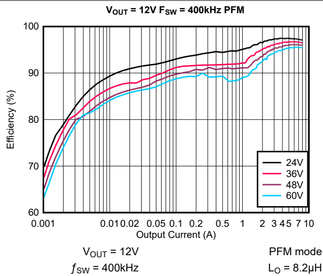
Figure 6-1. Efficiency PFM Mode
