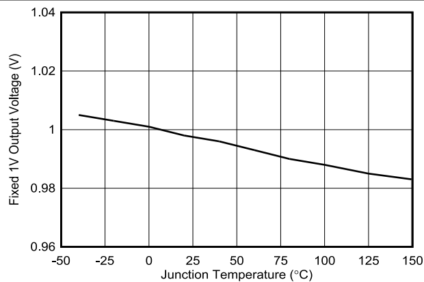
Figure 6-5. Fixed Output Voltage vs Temperature, V_{OUT} = 1\text{V}
