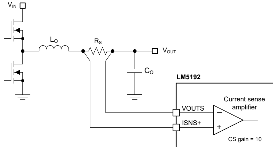
Figure 7-6. Shunt Current Sensing Implementation
