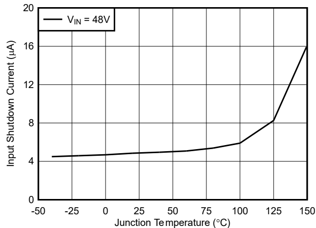
Figure 6-3. Input Shutdown Current vs Temperature
