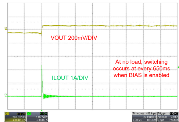
Figure 9-10. No Load Operation in PFM Mode, V_{SUPPLY} = 48V , I_{LOAD} = 0A
