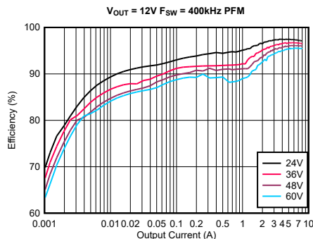
LM5192-Q1 Efficiency
