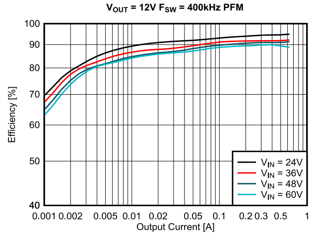
Figure 9-6. PFM Mode Efficiency, Log Scale
