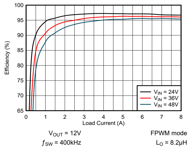
Figure 6-2. Efficiency FPWM Mode
