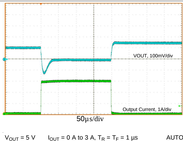
Figure 30. Load Transients
