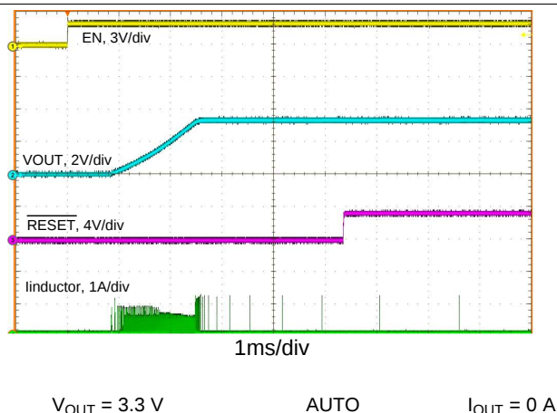
Figure 41. Start-up
