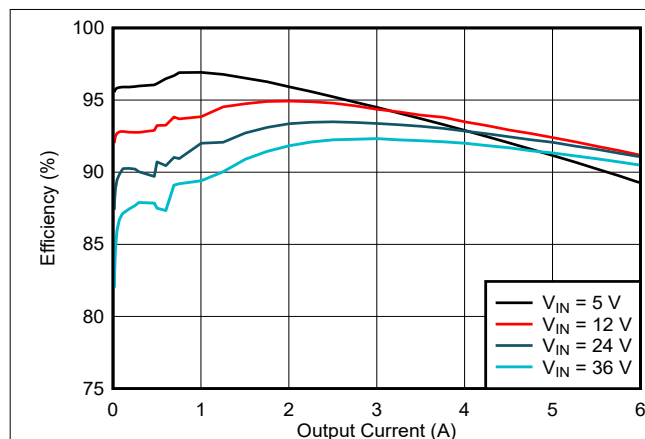
Figure 8-22. LM634x0-Q1 Efficiency
