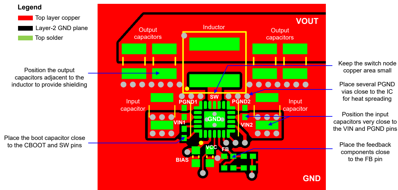
Figure 8-31. PCB Layout Example
