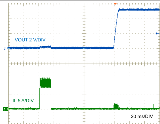
Figure 7-11. Short-Circuit Recovery
