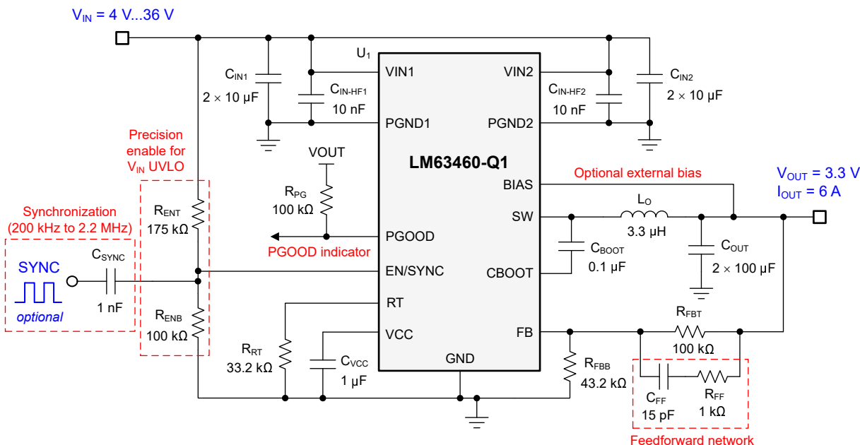
Figure 8-21. Application Circuit 3 – 3.3V, 6A at 400kHz
