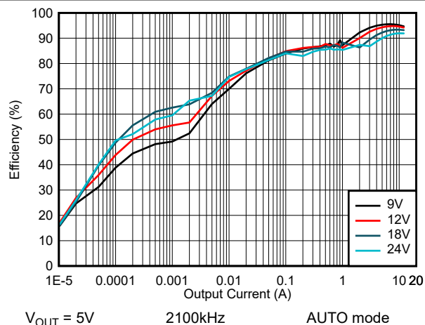
Figure 8-18. LM654A2 Efficiency
