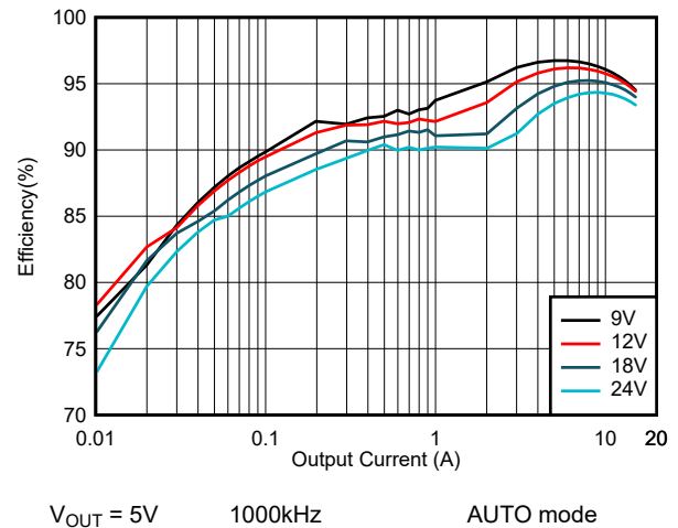
Figure 8-28. LM654A5 Efficiency
