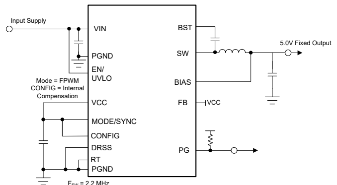
Simplified Schematic
