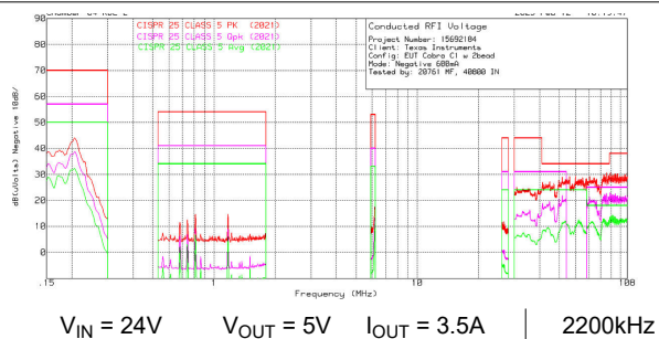
Figure 8-78. LM6x635 Conducted EMI - Negative Line
