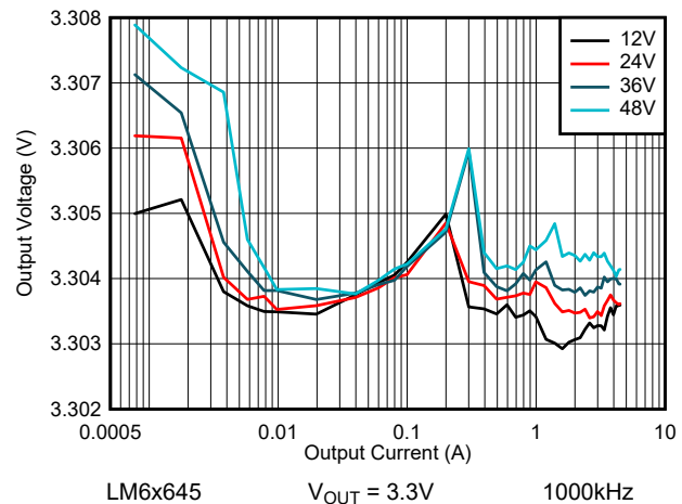
Figure 8-51. LM6x645 Line and Load Regulation - Auto Mode
