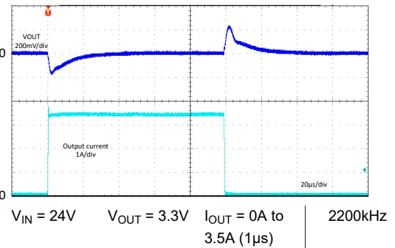
Figure 8-84. Load Transient - LM6x635 - FPWM
