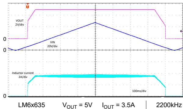
Figure 8-94. Line Sweep - Auto
