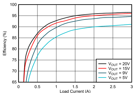
Typical Efficiency, V_{IN} = 48V , f_{SW} = 400kHz
