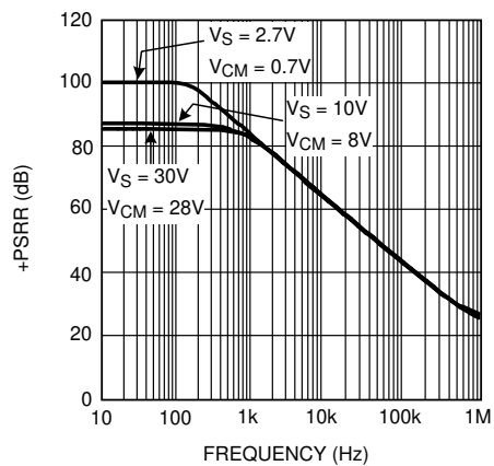
Figure 5-36. +PSRR vs Frequency, Old Die
