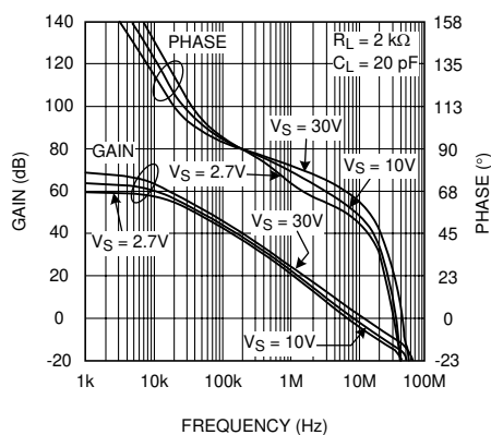
Figure 5-33. Open-Loop Frequency Response with Various Supply Voltage, Old Die
