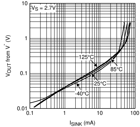
Figure 5-2. Output Swing vs Sinking Current, Old Die
