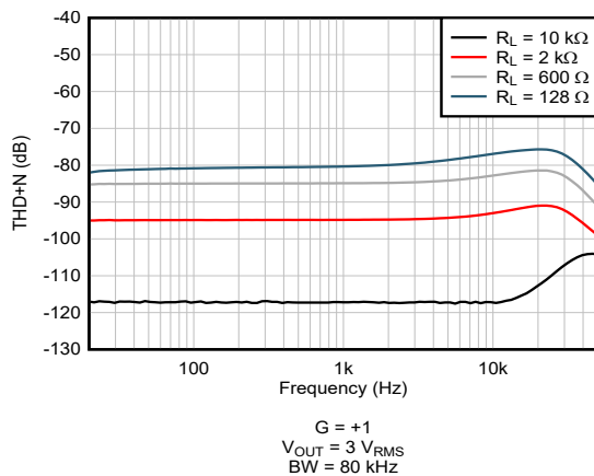
Figure 5-53. THD+N Ratio vs Frequency, New Die
