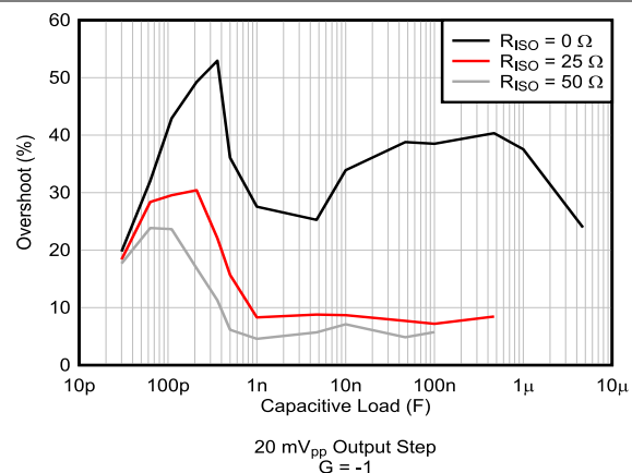
Figure 5-56. Small-Signal Overshoot vs Capacitive Load, New Die
