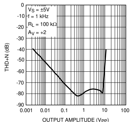
Figure 5-45. THD+N vs Output Amplitude, Old Die
