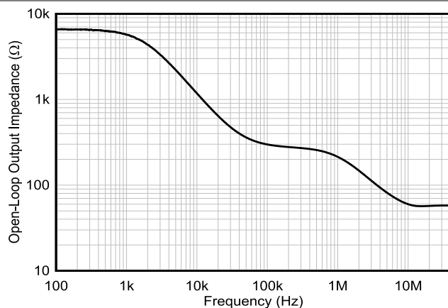
Figure 5-55. Open-Loop Output Impedance vs Frequency, New Die
