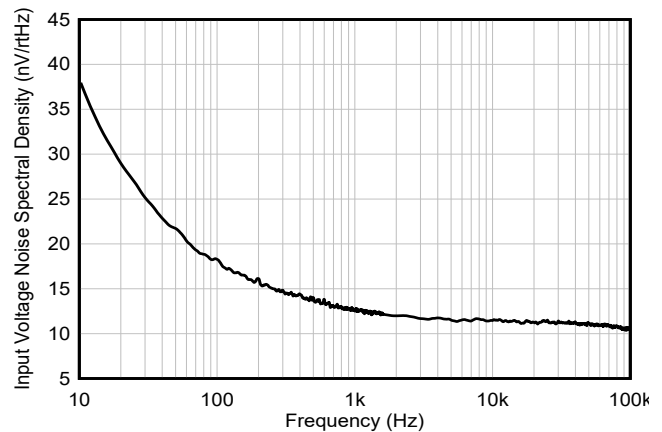
Figure 5-52. Input Voltage Noise Spectral Density vs Frequency, New Die
