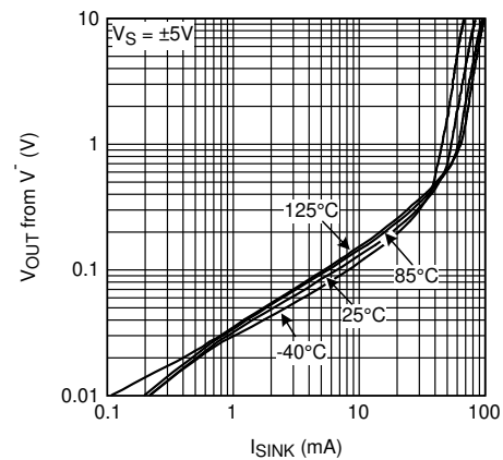
Figure 5-4. Output Swing vs Sinking Current, Old Die
