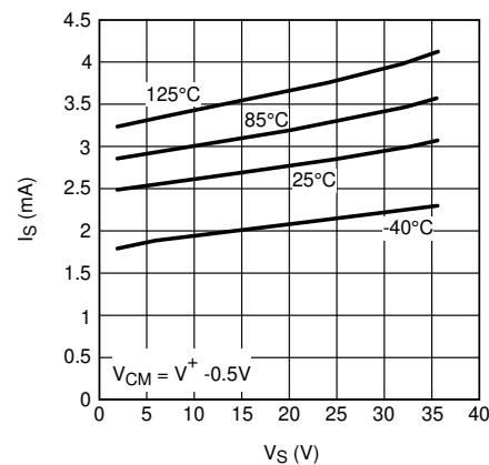
Figure 5-24. I_S vs (LM7322), Old Die
