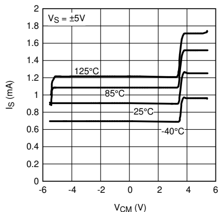
Figure 5-19. I_S vs V_{CM} (LM7321), Old Die
