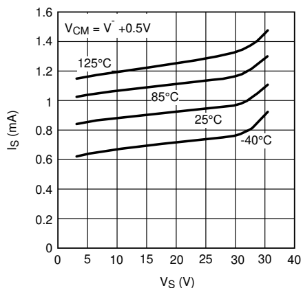
Figure 5-23. I_S vs (LM7321), Old Die
