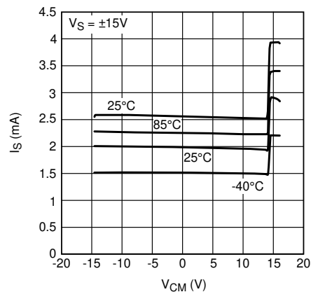
Figure 5-22. I_S vs V_{CM} (LM7322), Old Die
