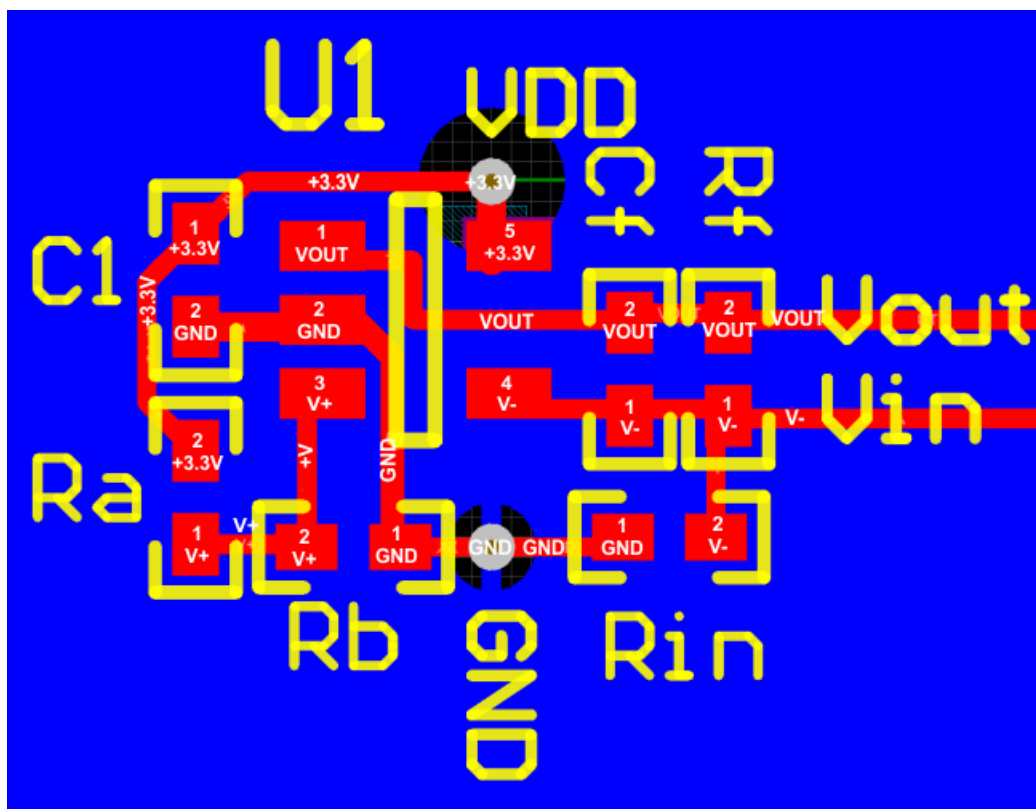
Figure 7-2. LM732xx Layout Example
