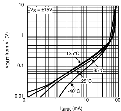
Figure 5-6. Output Swing vs Sinking Current, Old Die
