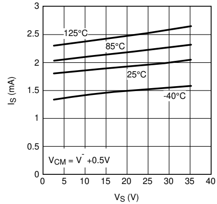
Figure 5-26. I_S vs (LM7322), Old Die
