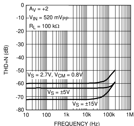
Figure 5-43. THD+N vs Frequency, Old Die
