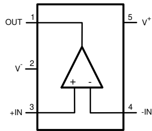
Figure 4-1. DBV Package 5-Pin SOT-23 Top View
