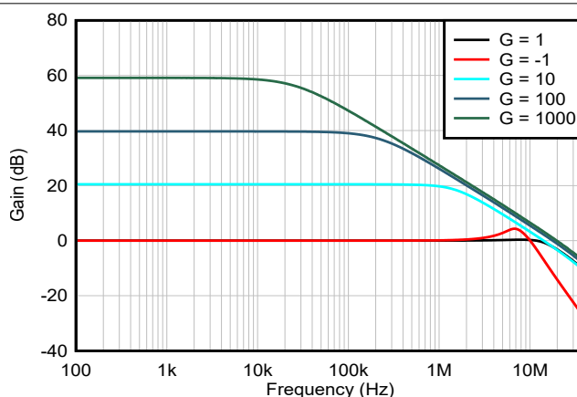
Figure 5-48. Closed-Loop Gain vs Frequency, New Die
