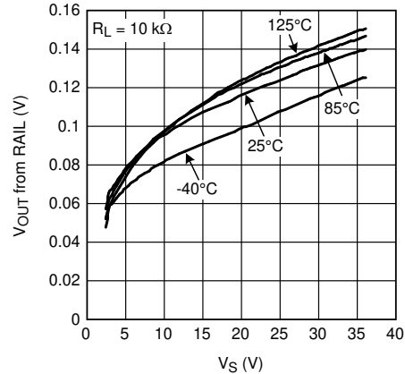
Figure 5-28. Positive Output Swing vs Supply Voltage, Old Die
