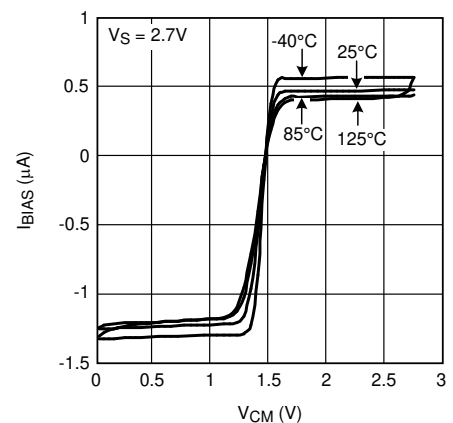
Figure 5-12. I_{BIAS} vs V_{CM} , Old Die
