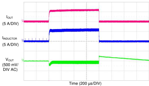
Figure 69. LM73606 Load Transients
