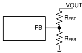
Figure 13. Output Voltage Setting by Resistor Divider
