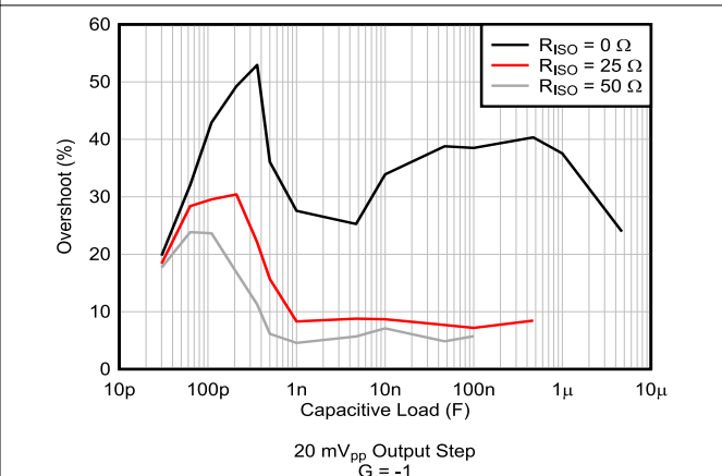
Figure 5-51. Small-Signal Overshoot vs Capacitive Load, New Die
