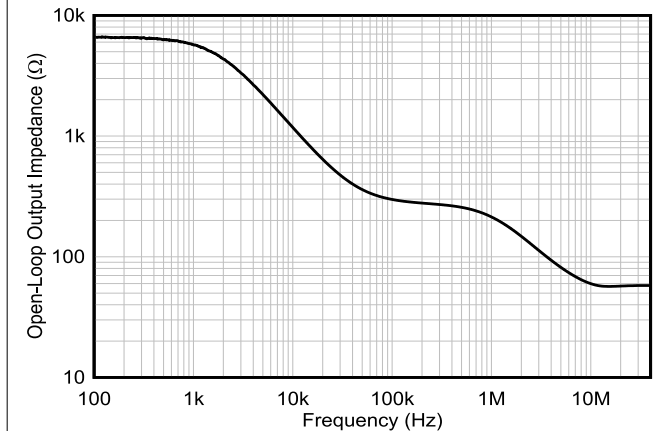
Figure 5-50. Open-Loop Output Impedance vs Frequency, New Die
