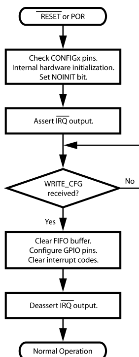
Figure 4. LM8323 Initialization Behavior
