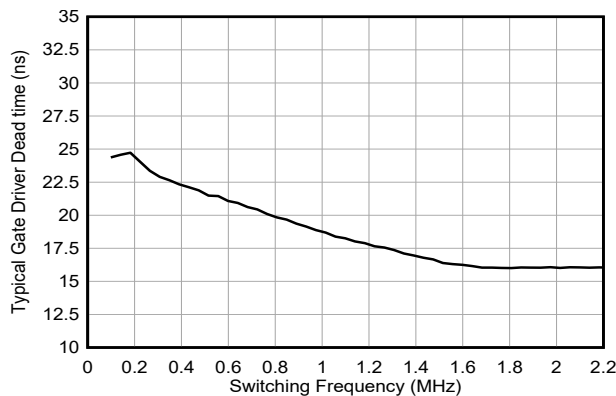
Figure 6-23. Gate Driver Transition (Dead) Time Versus Switching Frequency \text{SEL\_MIN\_DEADTIME\_GDRV} = 0b01, \text{SEL\_SCALE\_DT} = 0b0, \text{EN\_CONST\_TDEAD} = 0b0
