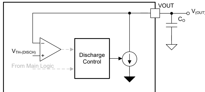
Figure 8-14. Functional Block Diagram Output Discharge
