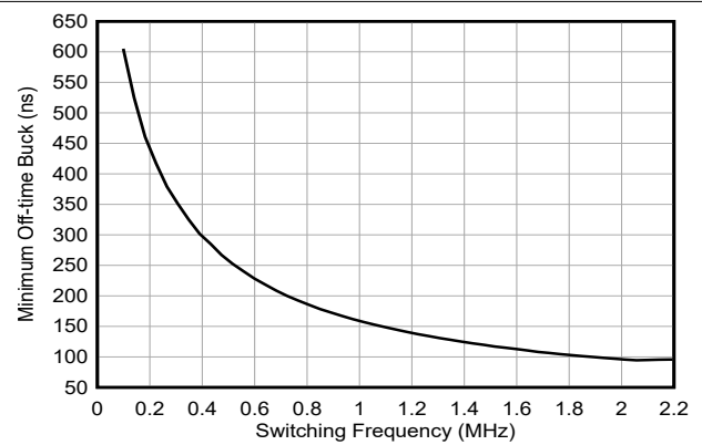
Figure 6-18. Buck Minimum Off-time Versus Switching Frequency
