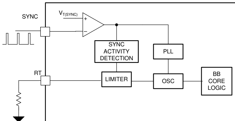
Figure 8-20. Main Oscillator Functional Block Diagram
