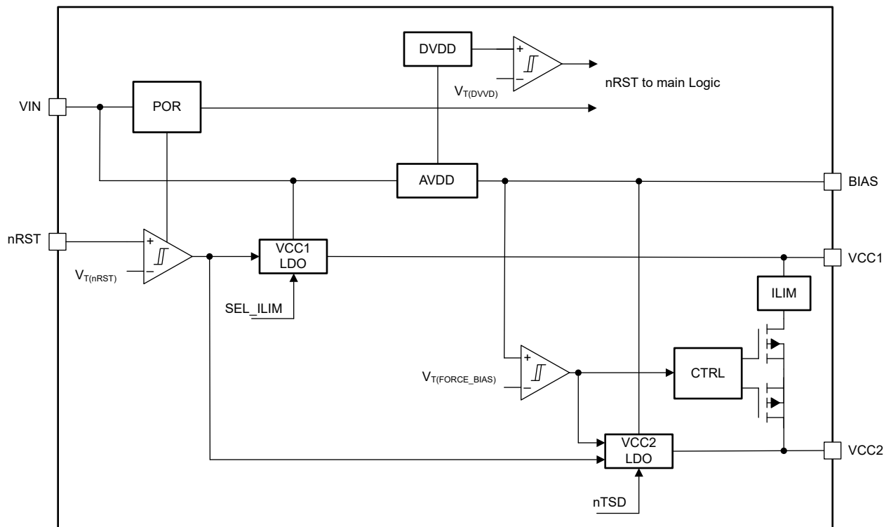
Figure 8-8. Functional Block Diagram Reference System
