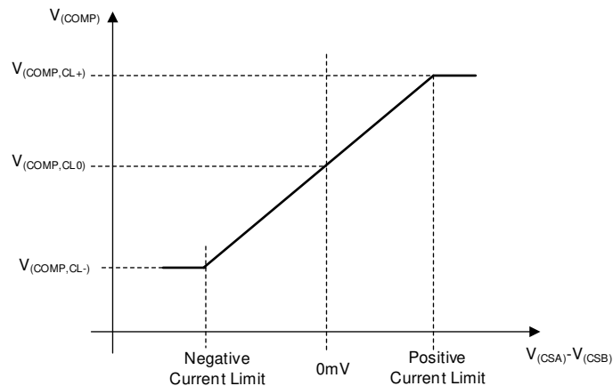
Figure 8-12. Control Function for the Peak Current Sense Voltage Versus V_{COMP}
