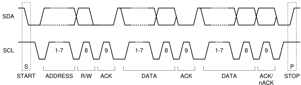
Figure 8-31. I 2 C START / STOP / ACKNOWLEDGE Protocol
