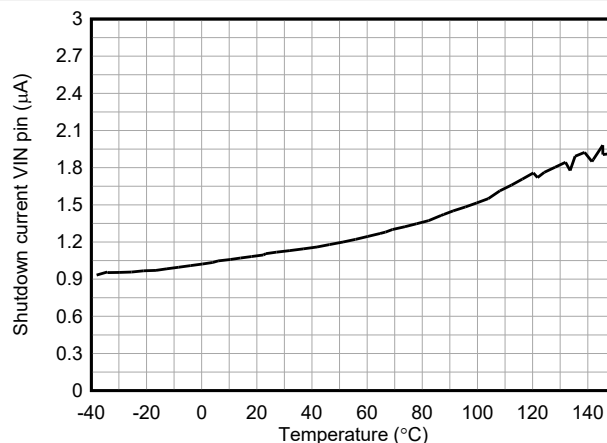
Figure 6-6. Shutdown Current Into VIN Versus Temperature V_{EN/UVLO} = 0\text{V} , V_{(VIN)} = 12\text{V} , V_{(BIAS)} = 0\text{V}
