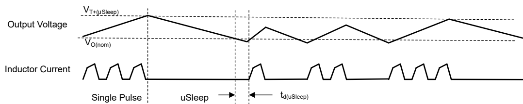
Figure 8-6. Timing Diagram for the Power Save Mode (μSleep Enabled)
