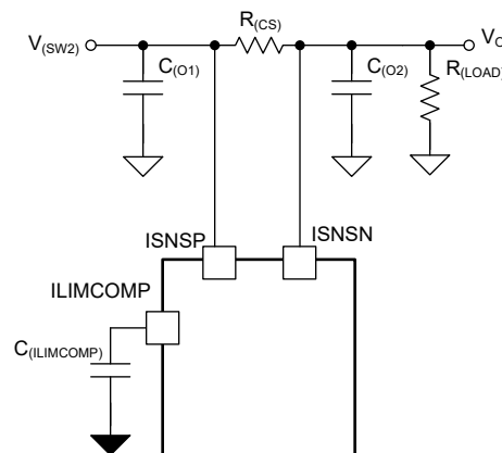
Figure 8-17. Simplified Schematic Current Limit Components With Resistive Load
