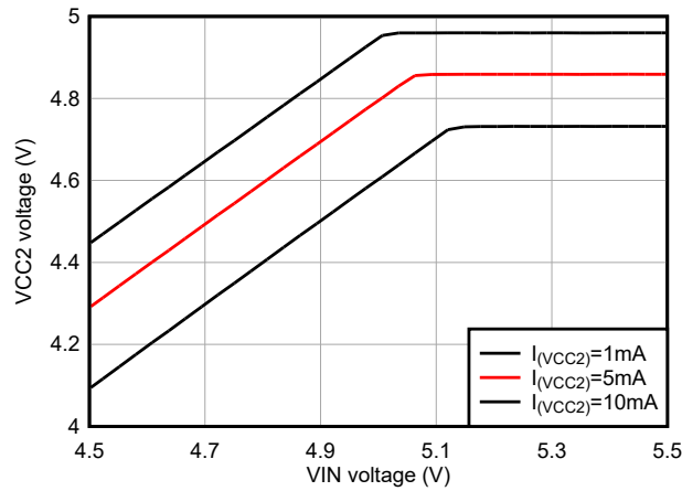
Figure 6-13. VCC2 LDO Output Voltage Versus VIN Voltage V_{(BIAS)} = 0\text{V}
