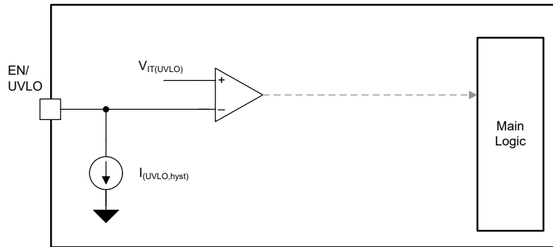
Figure 8-11. Functional Block Diagram UVLO
