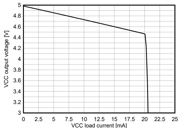
Figure 6-11. VCC2 LDO Output Voltage Versus VCC2 Load Current V_{(VIN)} = 12\text{V} , V_{(BIAS)} = 0\text{V}
