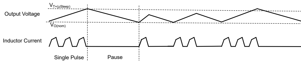
Figure 8-5. Timing Diagram for the Power Save Mode (μSleep Disabled)
