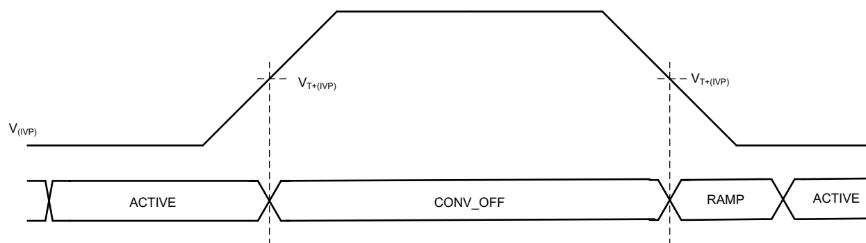
Figure 8-29. Timing Diagram IVP Operation
