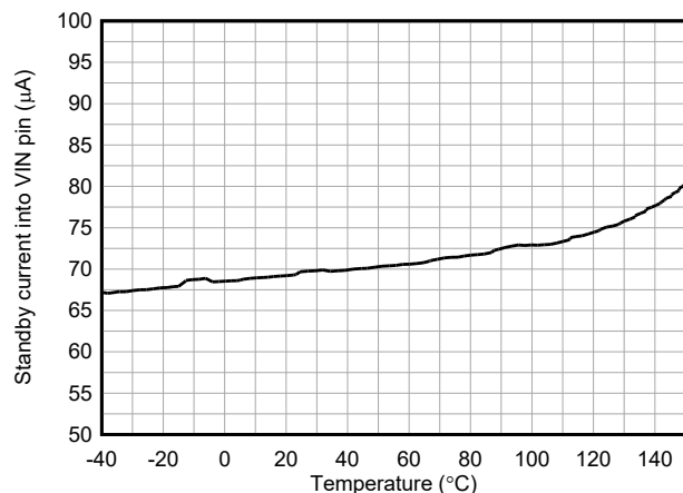
Figure 6-10. Standby Current Into VIN Versus Temperature V_{(BIAS)} = 3.5\text{V} , V_{(VIN)} = 12\text{V}
