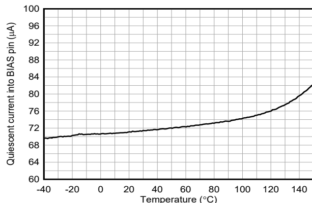
Figure 6-9. Quiescent Current Into BIAS Versus Temperature V_{(BIAS)} = 12\text{V} , V_{(VIN)} = 3.5\text{V}
