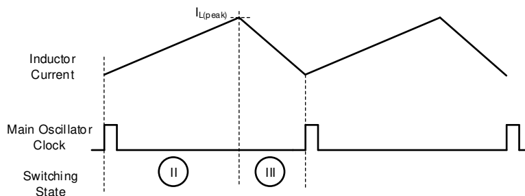
Figure 8-2. Inductor Current in Continuous Current Buck Operation
