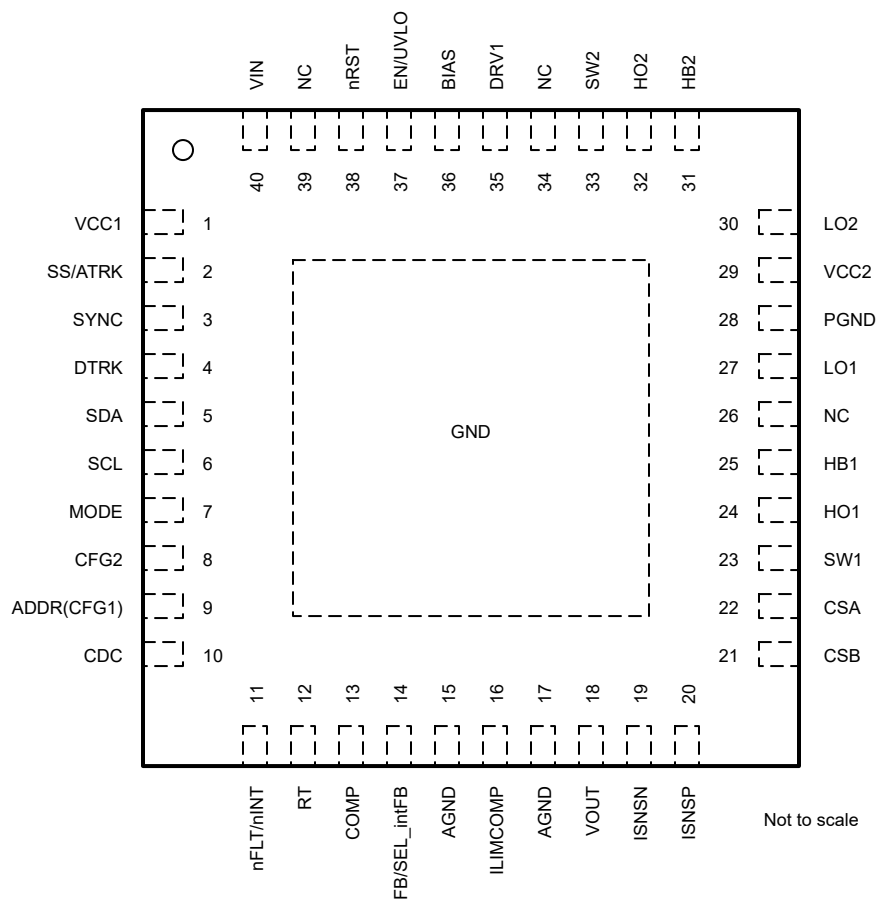
Figure 5-1. LM851772-Q1 RHA Package, 40-Pin VQFN (Top View)
