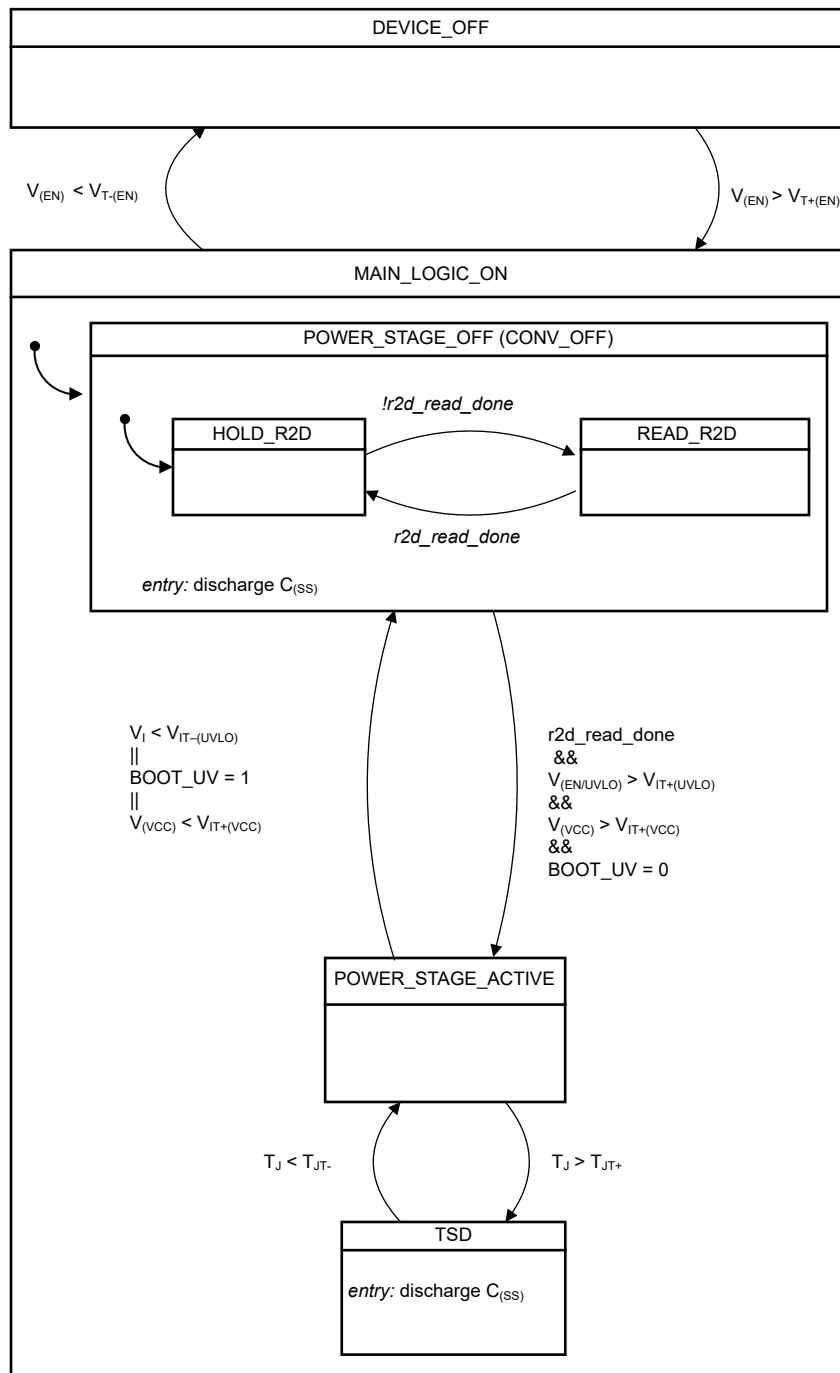
Figure 8-30. State Diagram
