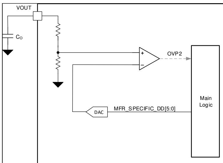
Figure 8-28. Functional Block Diagram OVP2
