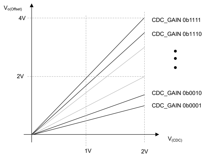
Figure 8-26. Vo Offset vs CDC Voltage
