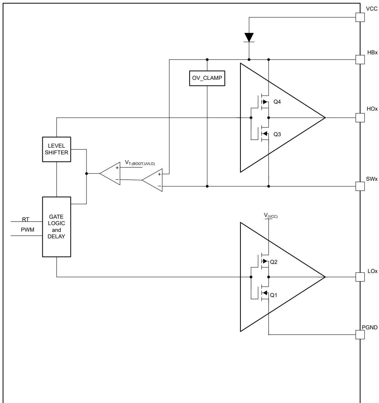
Figure 8-25. Functional Block Diagram Gate Driver
