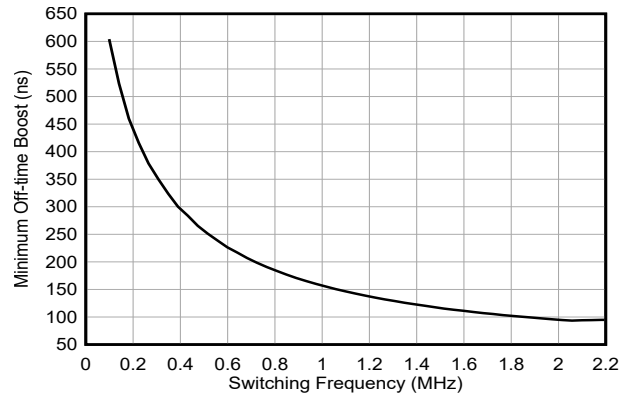
Figure 6-20. Boost Minimum Off-time Versus Switching Frequency
