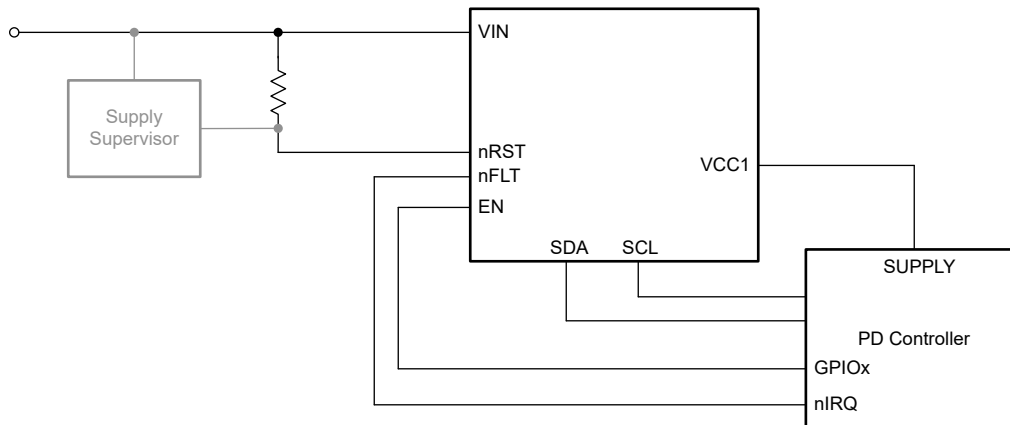
Figure 8-9. Simplified Schematic
