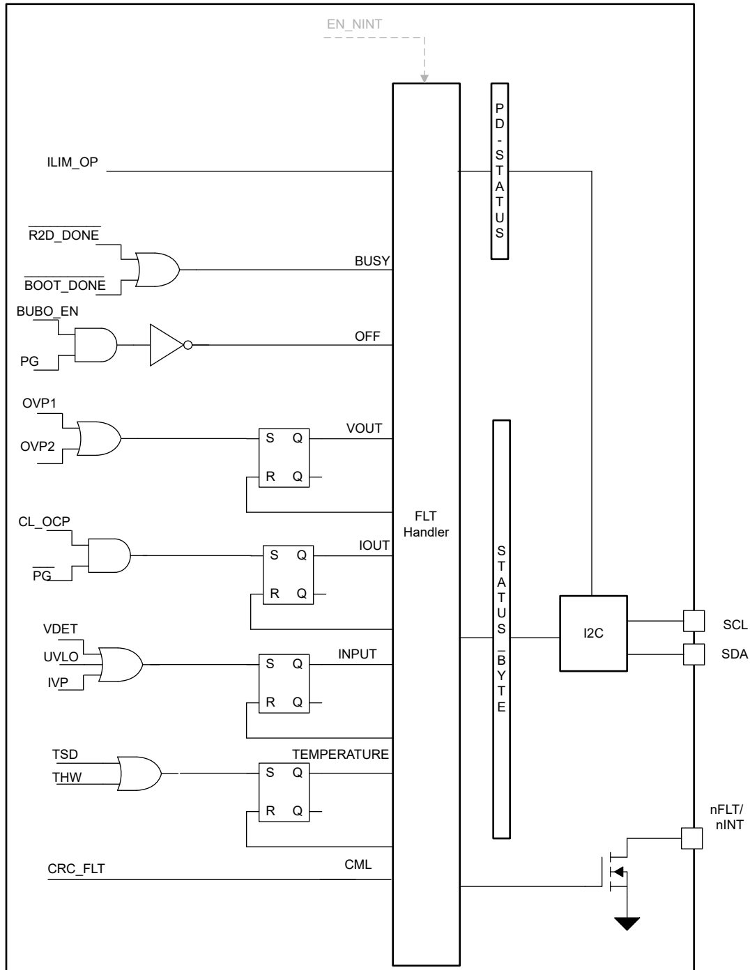
Figure 8-27. Functional Block Diagram Fault Handler
