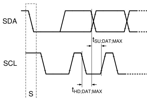
Figure 8-33. I 2 C Data Transmission Timing for Maximum Rise and Fall Times
