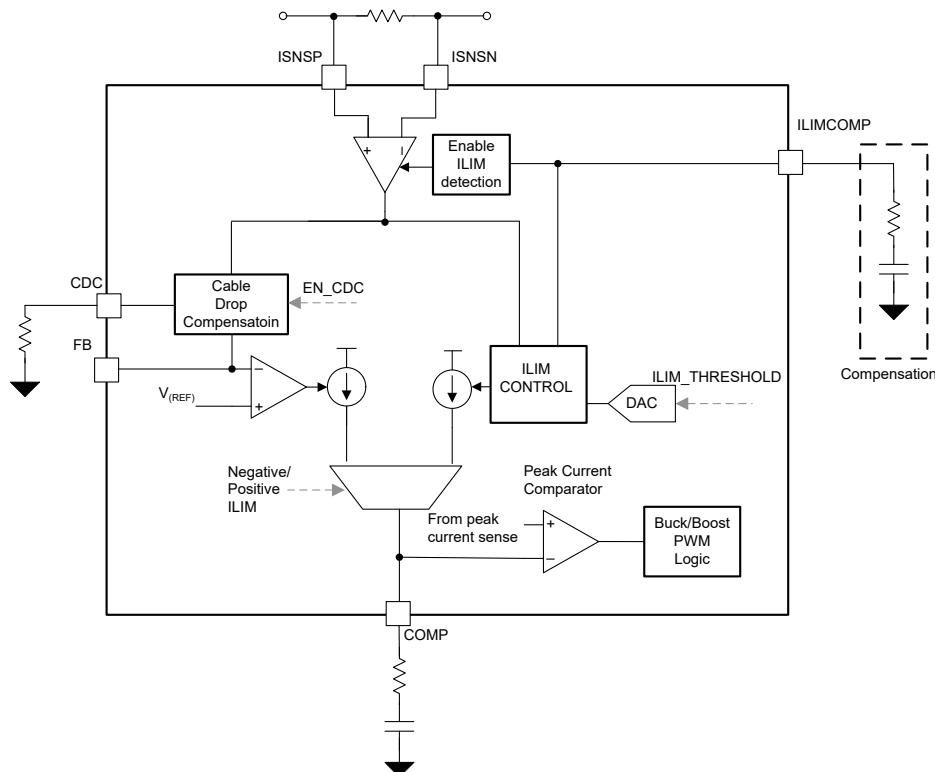
Figure 8-16. Current Monitor Functional Block Diagram
