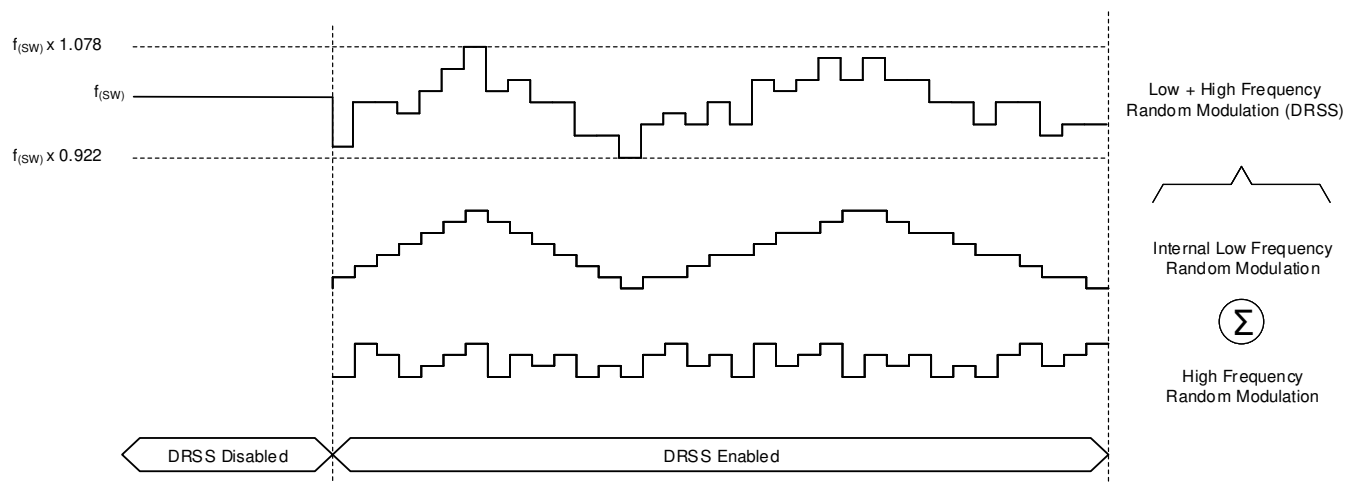
Figure 8-24. Dual Random Spread Spectrum
