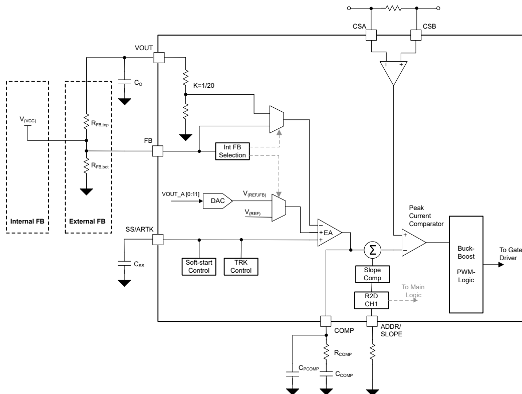
Figure 8-13. EA Functions Block Diagram
