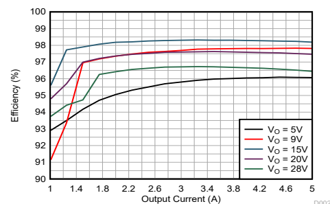
Efficiency vs Output Current, V_I = 12V , PSM
