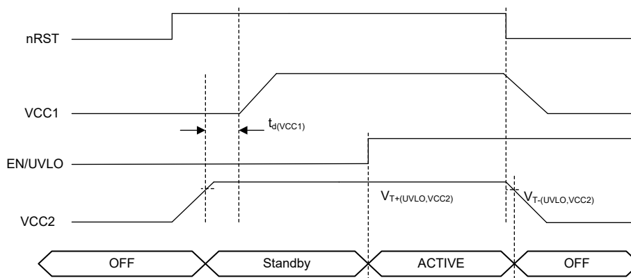
Figure 8-10. Timing Diagram VCC Regulator V_{(BIAS)} > V_{T+(Sel,BIAS)}
