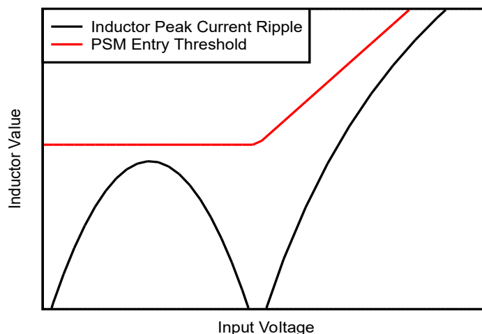
Figure 8-7. Generic Graph of PSM Entry Threshold And Ripple Current Versus Input Voltage
