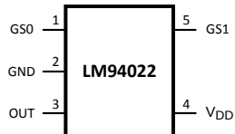
Pin Functions
