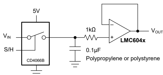
Figure 6-7. Low-Leakage Sample and Hold
