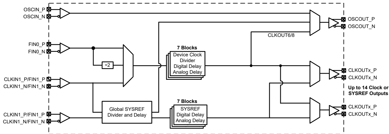
Figure 8-15. Simplified Functional Block Diagram for Distribution Mode
