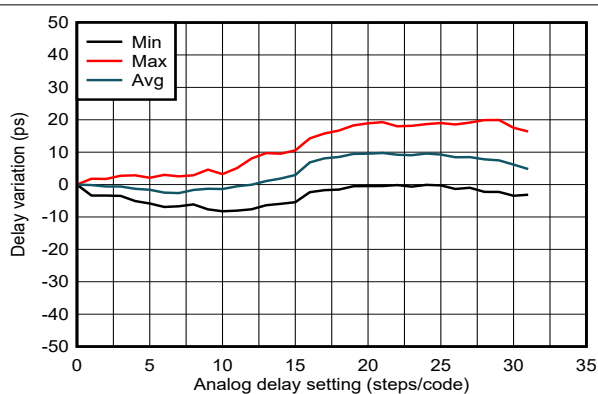
Figure 6-22. SYSREF/1PPS Delay Linearity vs. Analog Delay Code 3
