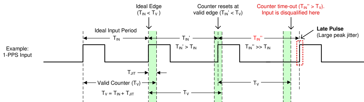
Figure 7-19. 1PPS Input Window Detector Example
