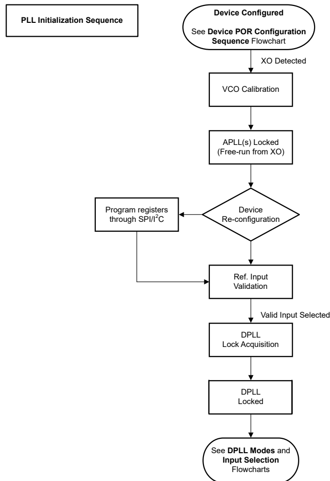
Figure 7-42. APLL Initialization Sequence
