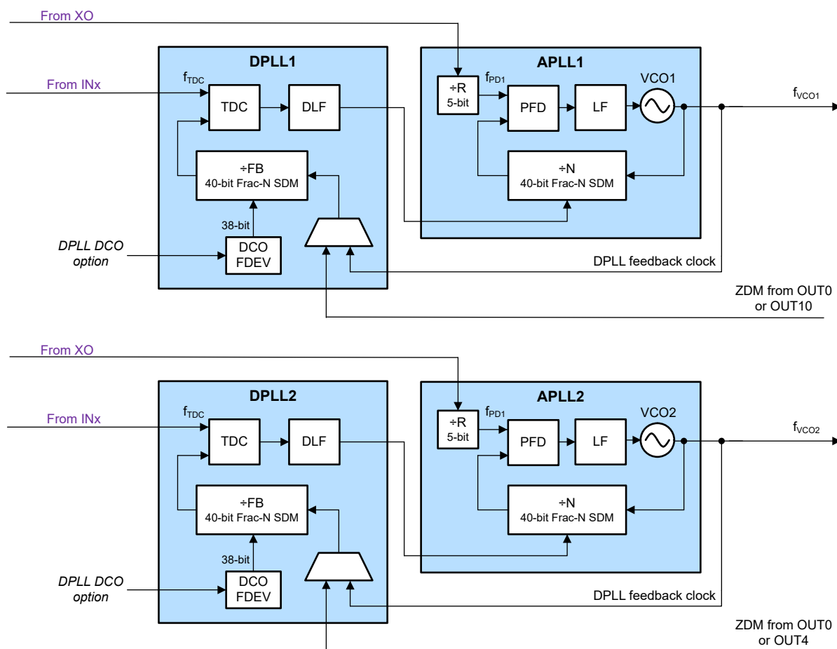
Figure 7-3. DPLL Operation
