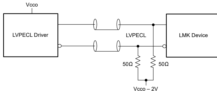
Figure 7-11. DC-Coupled LVPECL to Reference (INx)
