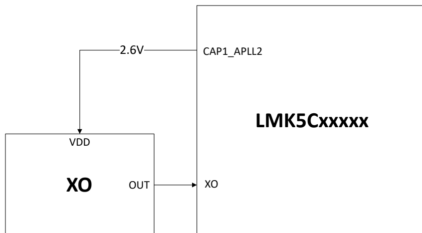
Figure 8-3. Supplying XO Input with CAP1_APLL2
