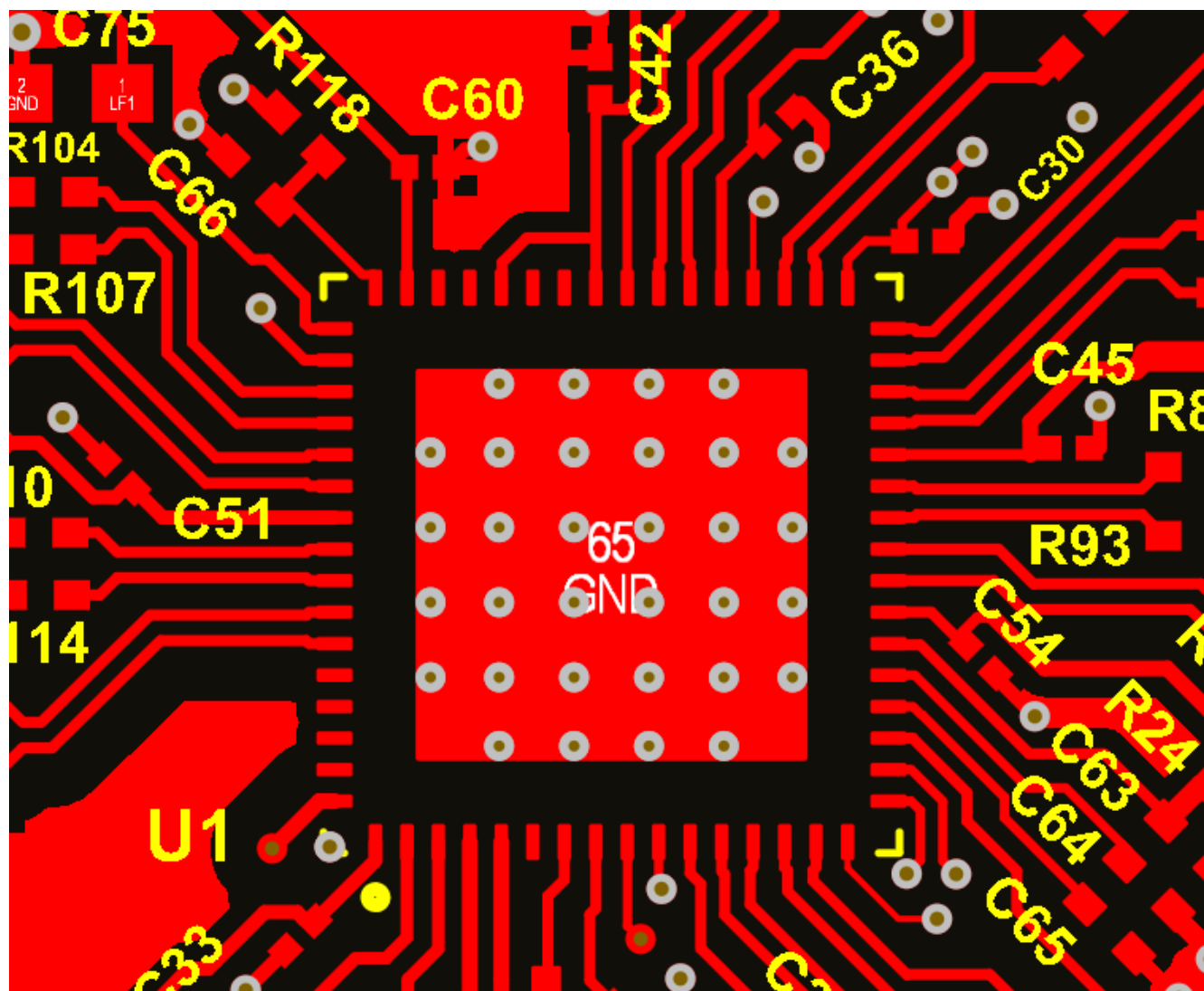
Figure 8-6. PCB Layout Example for LMK5C22212A , Top Layer
