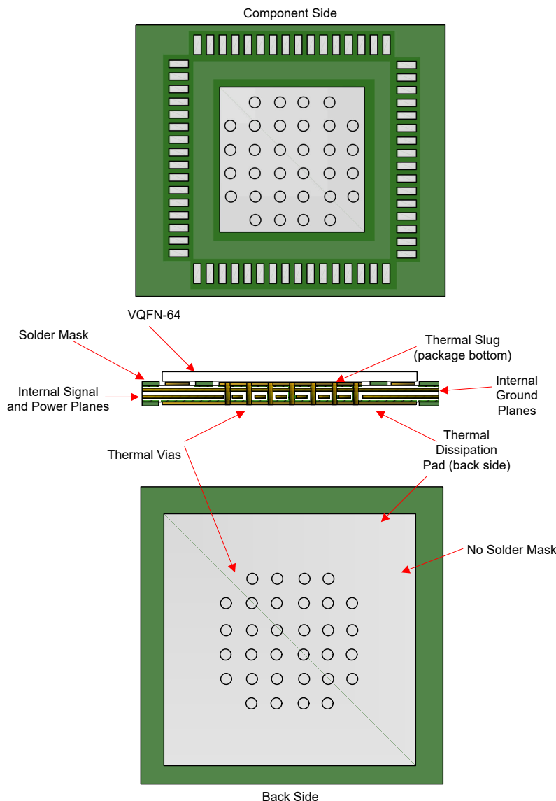
Figure 8-8. General PCB Ground Layout for Thermal Reliability (8+ Layers Recommended)
