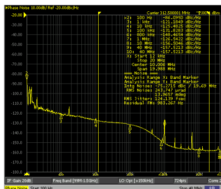
Figure 5-12. 312.5MHz HSDS Output From APPL2
