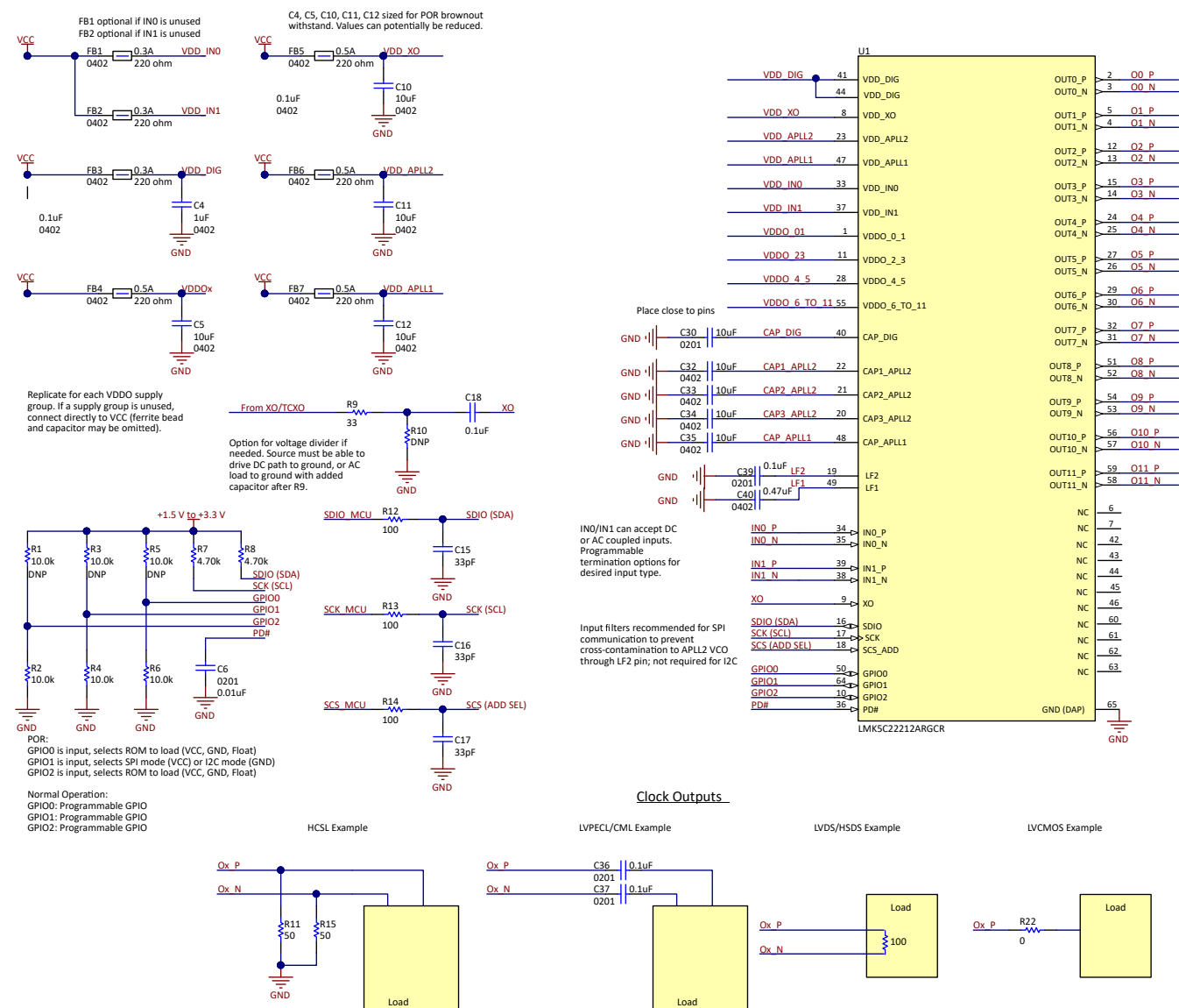
Figure 8-4. Reference Schematic Example
