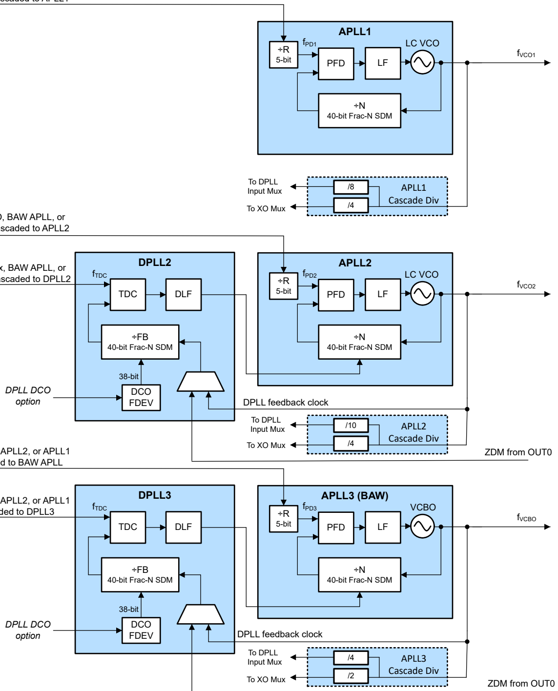
Figure 8-2. PLL Architecture
