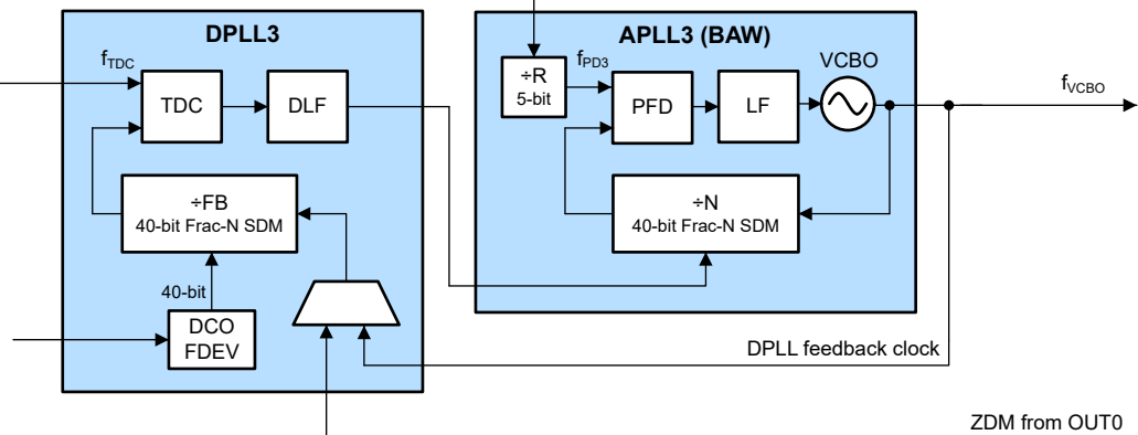
Figure 8-6. APLL Cascaded With DPLLs Disabled Example
