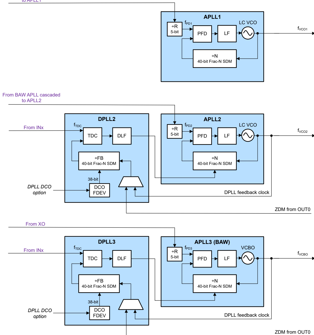
Figure 8-5. APLL Cascaded With DPLLs Enabled Example
