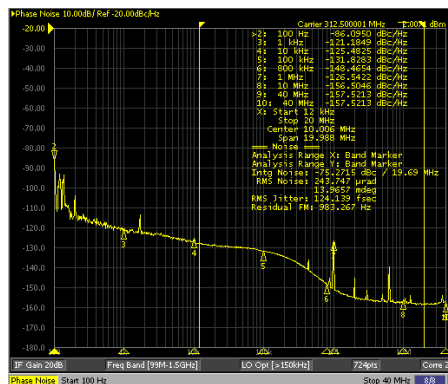
Figure 6-12. 312.5MHz HSDS Output From APPL2
