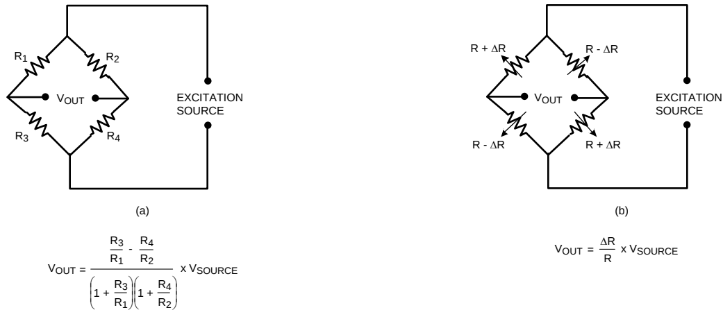
Figure 51. Bridge Sensor
