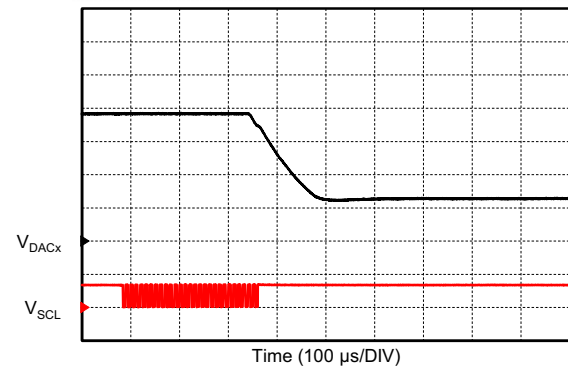
Figure 16. DAC Step Response DAC OVERRIDE MODE C_L = 10\text{ pF} I^2\text{C} command triggers DAC step Step size: 3/4 to 1/4 FS
