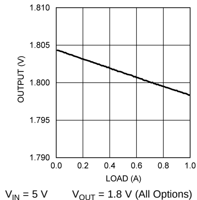
Figure 19. Load Regulation
