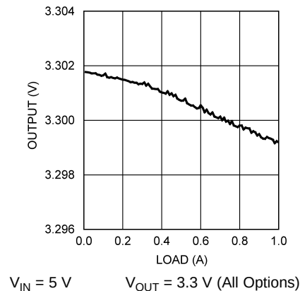
Figure 20. Load Regulation
