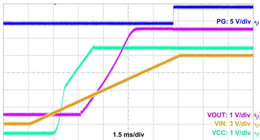
Figure 8-5. Typical Start-up Behavior V_{IN} = 12\text{ V} , V_{OUT} = 5\text{ V} , I_{OUT} = 1.5\text{ A}
