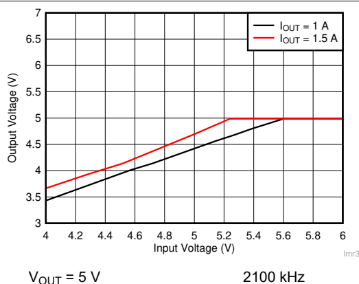
Figure 9-7. Overall Dropout Curve
