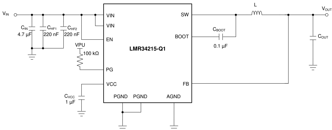
Figure 9-2. Example Applications Circuit (Fixed 5-V Output)
