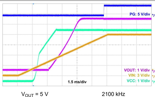
Figure 9-9. Start-Up Waveform
