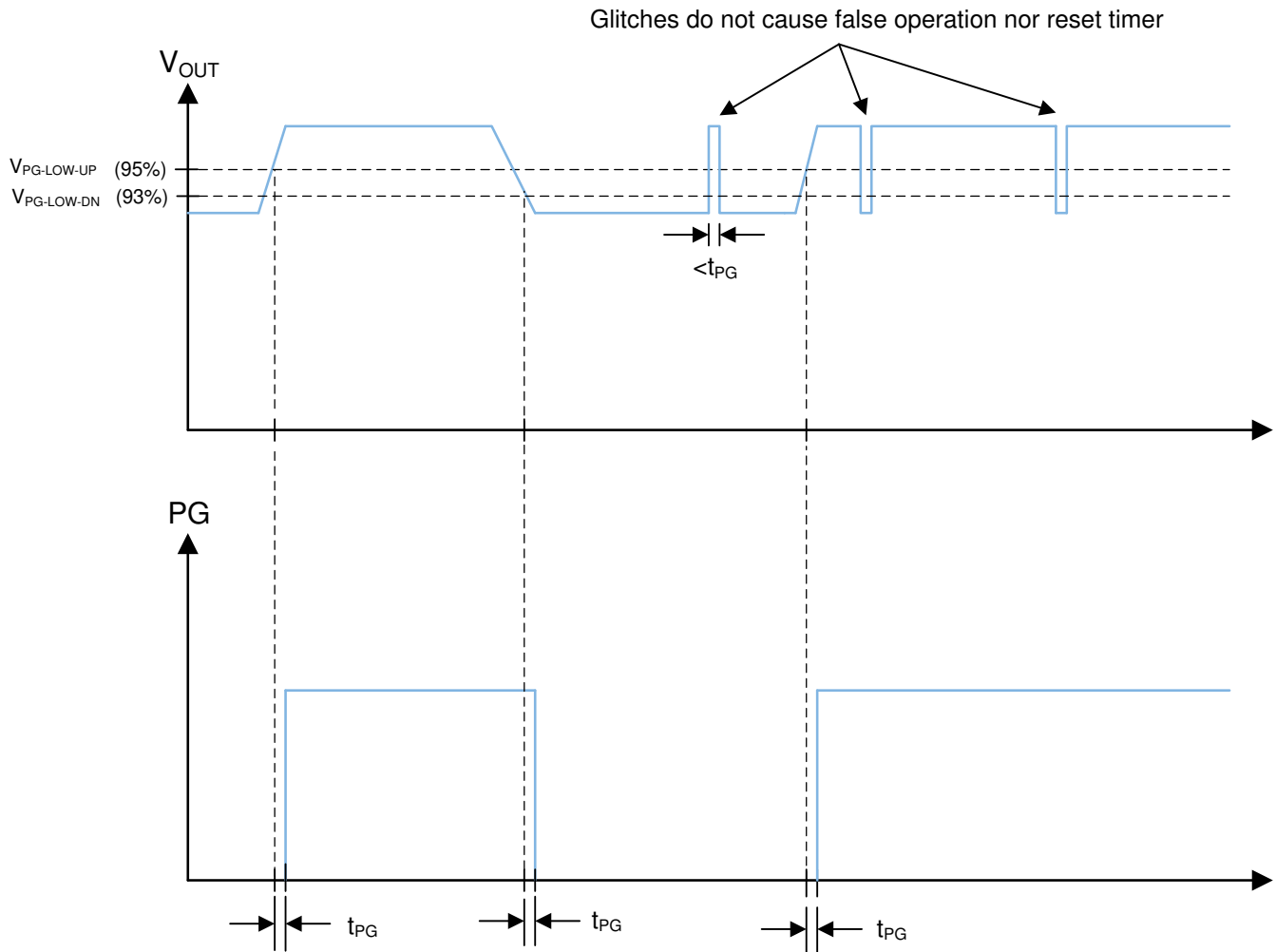
Figure 8-3. Power-Good-Timing Behavior
