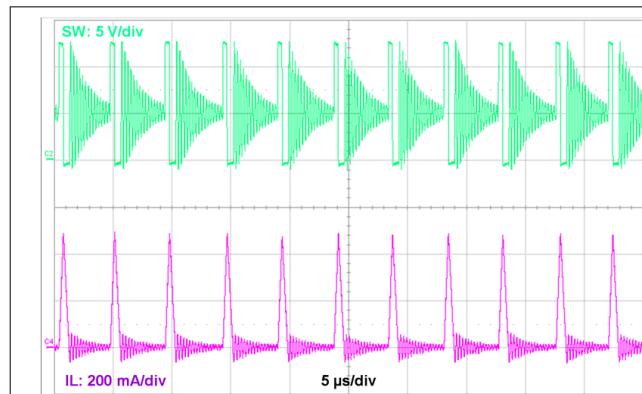
Figure 8-7. Typical PWM Switching Waveforms V_{IN} = 12\text{ V} , V_{OUT} = 5\text{ V} , I_{OUT} = 30\text{ mA} , f_S = 2100\text{ kHz}
