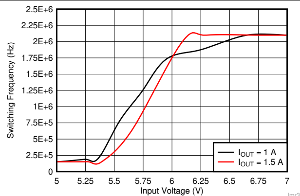
Figure 8-10. Typical f_{SW} vs Output Current f_{SW} = 2100 kHz
