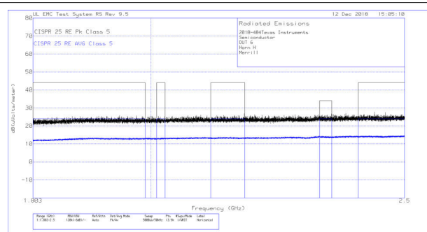
Figure 9-17. Radiated EMI Log Horizontal vs. CISPR25 Limits
