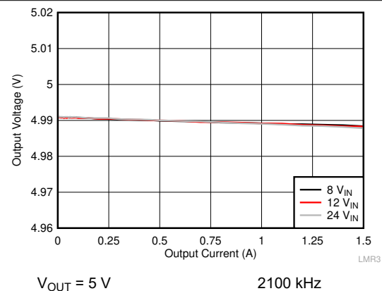
Figure 9-6. Load Regulation
