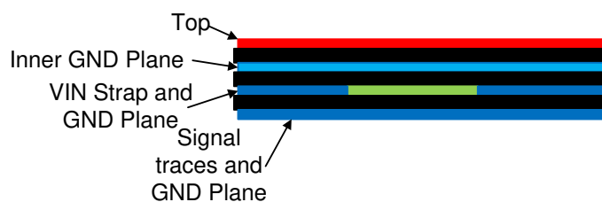
Figure 10-3. Example Layout for 400kHz, Adjustable Output
