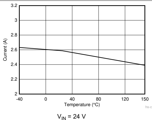
Figure 7-3. High Side Current Limit
