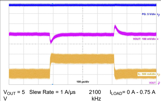
Figure 9-10. Load Transient Waveform
