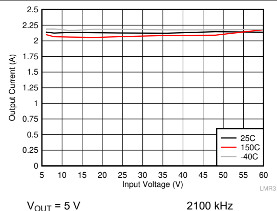
Figure 9-8. Load Current to Trigger Short Circuit
