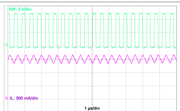
Figure 8-8. Typical PWM Switching Waveforms V_{IN} = 12\text{ V} , V_{OUT} = 5\text{ V} , I_{OUT} = 1.5\text{ A} , f_S = 2100\text{ kHz}
