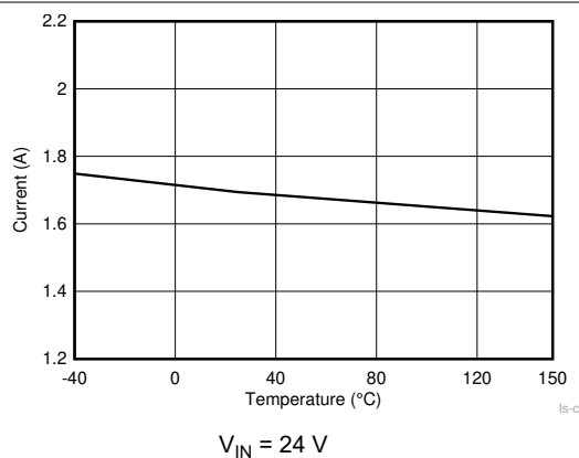
Figure 7-4. Low Side Current Limit
