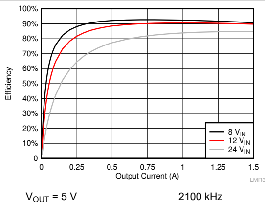
Figure 9-5. Efficiency
