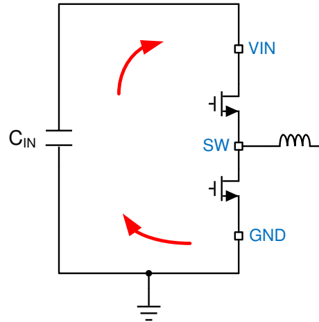
Figure 10-1. Current Loops with Fast Edges
