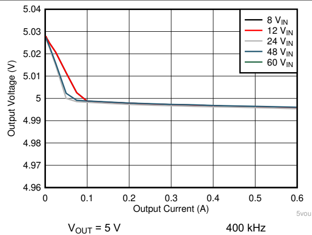
Figure 9-7. Load Regulation
