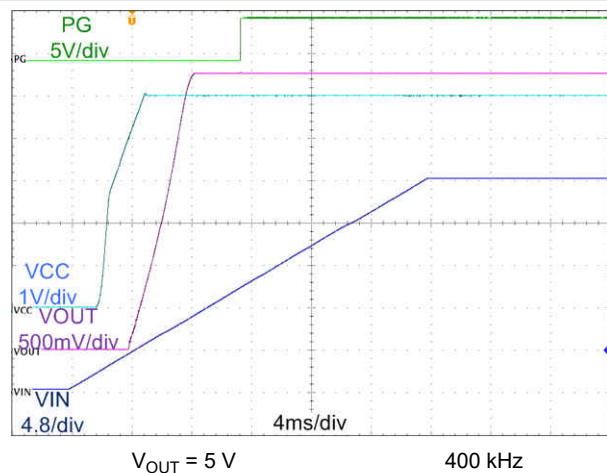
Figure 9-14. Start-Up Waveform
