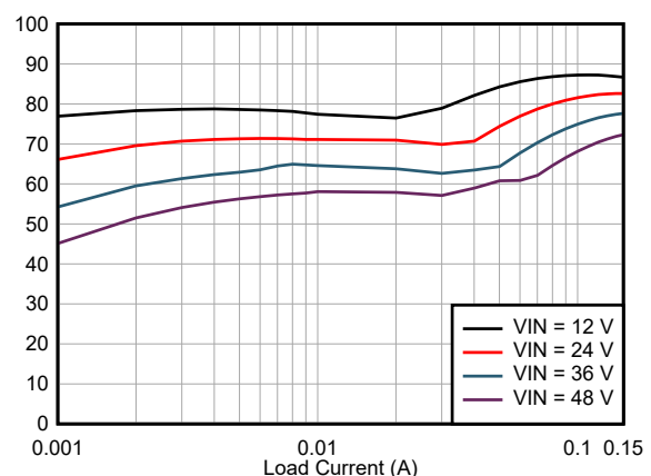
Efficiency versus Output Current V_{OUT} = 3.3\text{ V (Fixed)}, 1\text{ MHz, AUTO}
