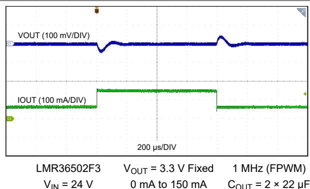
Figure 9-8. Load Transient
