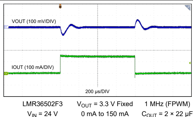
Figure 9-7. Load Transient
