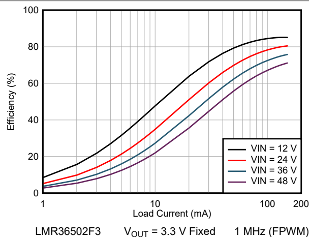
Figure 9-3. Efficiency
