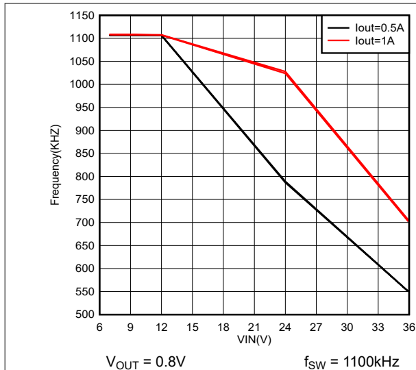
Figure 7-4. Frequency Foldback at T_{ON\_MIN}
