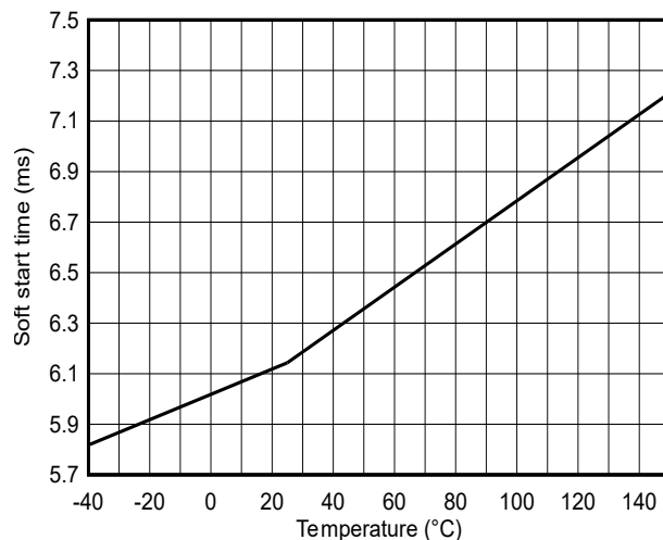
Figure 6-6. Soft-start time
