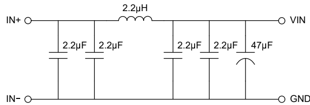
Figure 8-42. Recommended input EMI filter
