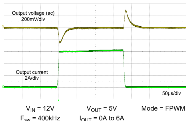
Figure 8-25. Load Transient
