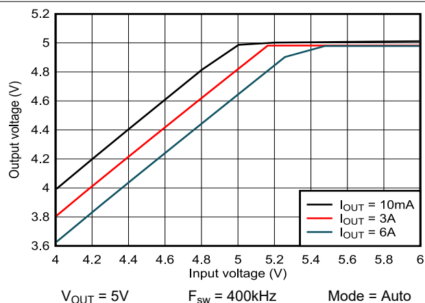
Figure 8-19. Dropout Curve
