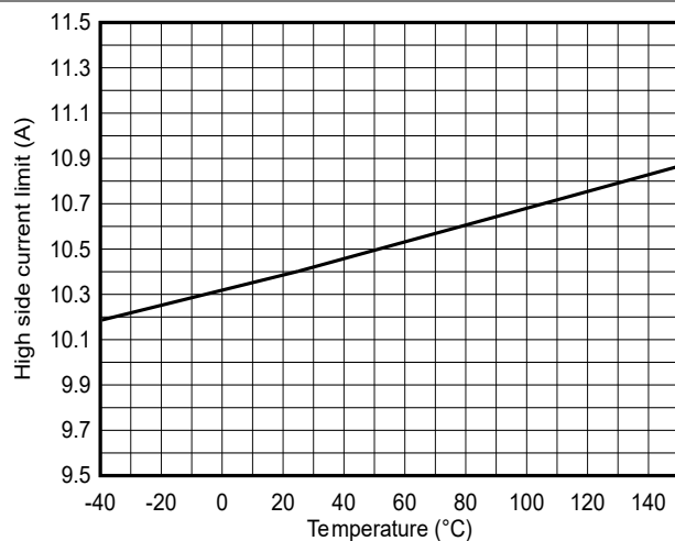
Figure 6-1. High-side MOSFET current limit
