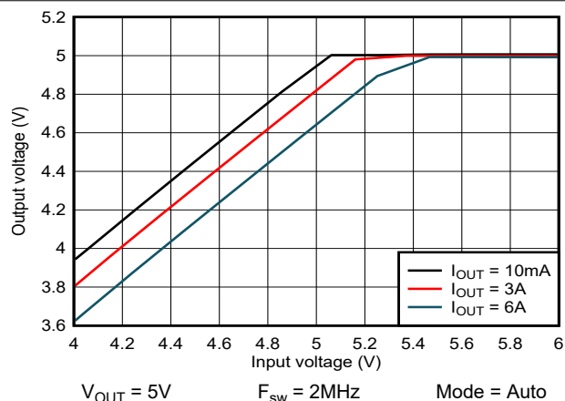
Figure 8-21. Dropout Curve
