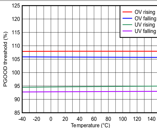
Figure 6-10. PGOOD thresholds
