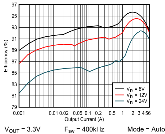
Figure 8-2. Efficiency - Auto Mode
