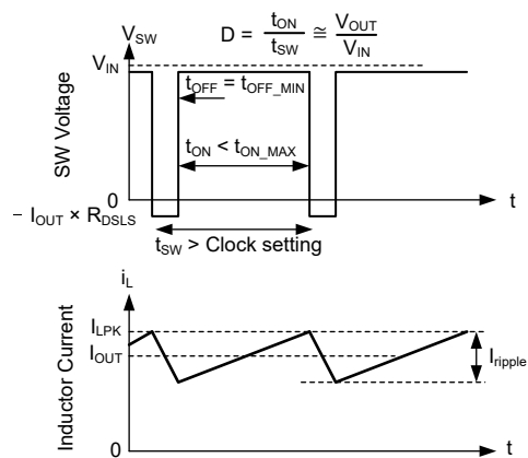
Figure 7-11. Dropout Waveforms
