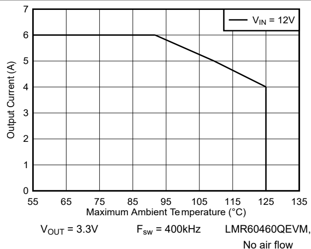
Figure 8-22. Output Current versus Maximum Ambient Temperature
