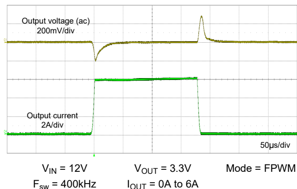
Figure 8-24. Load Transient
