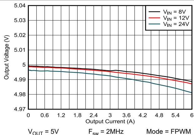
Figure 8-17. Load and Line Regulation - FPWM Mode
