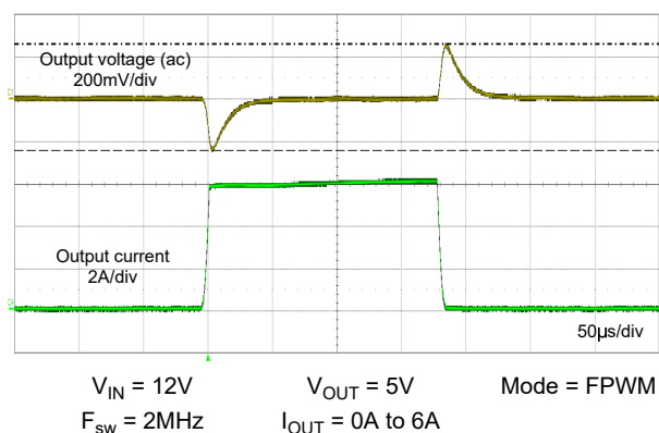
Figure 8-27. Load Transient
