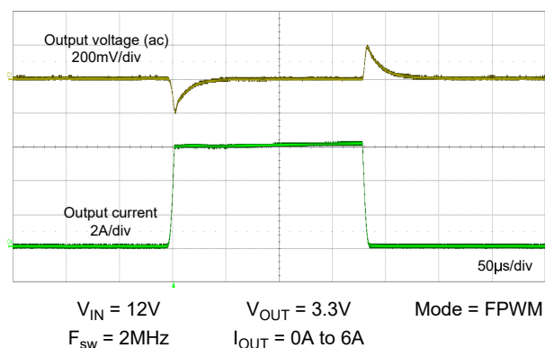
Figure 8-26. Load Transient
