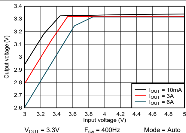
Figure 8-18. Dropout Curve
