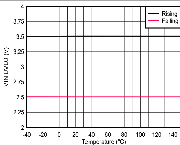
Figure 6-9. Input voltage UVLO
