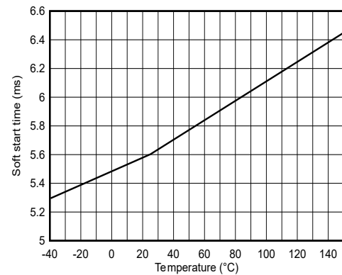
Figure 6-6. Soft-Start Time
