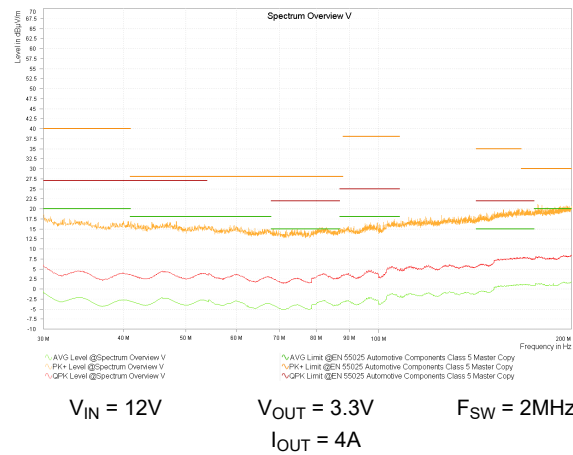
Figure 8-17. Radiated EMI (Bicon Vertical) vs CISPR 25 Limits
