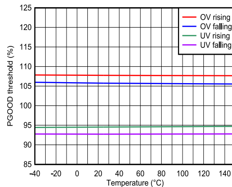
Figure 6-10. PGOOD Thresholds
