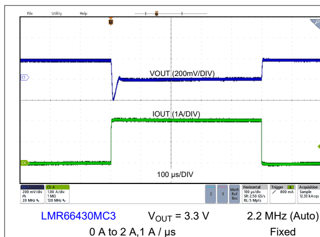
Figure 8-10. Load Transient
