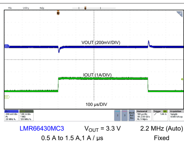
Figure 8-11. Load Transient
