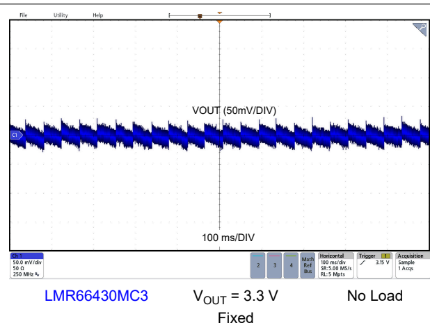
Figure 8-15. Output Voltage Ripple
