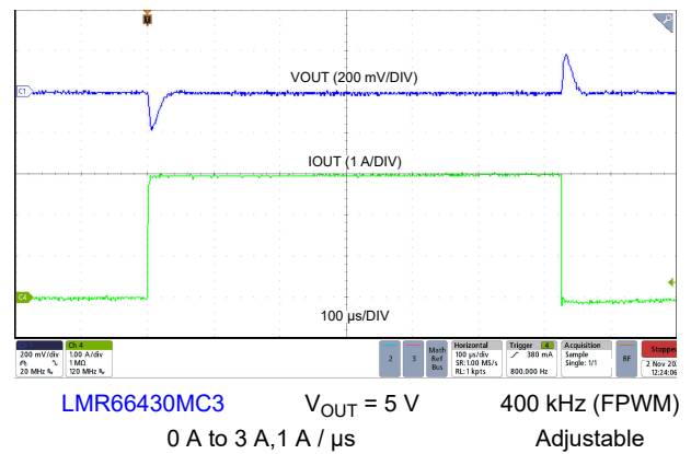
Figure 8-23. Load Transient
