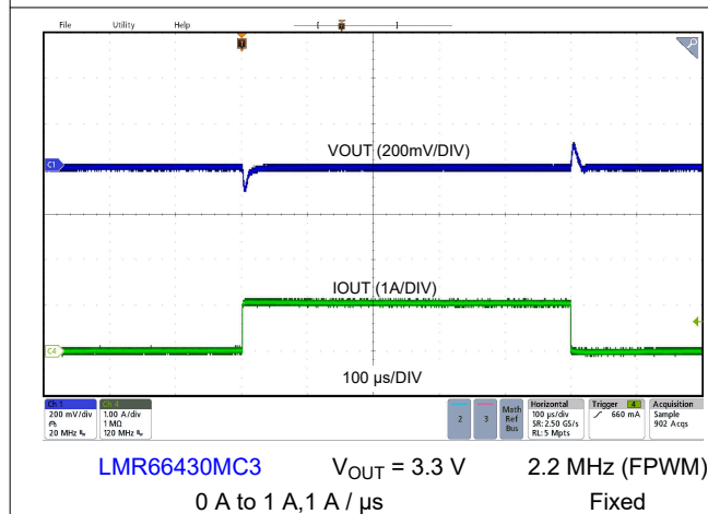
Figure 8-12. Load Transient
