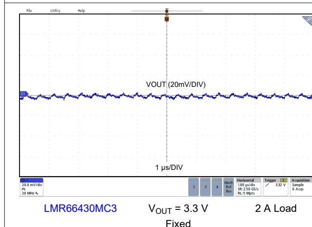
Figure 8-14. Output Voltage Ripple
