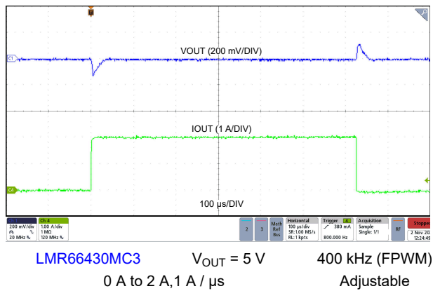
Figure 8-24. Load Transient
