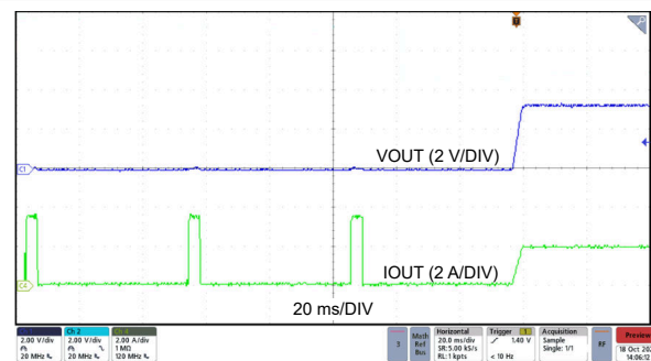
Figure 7-15. Hiccup Exit
