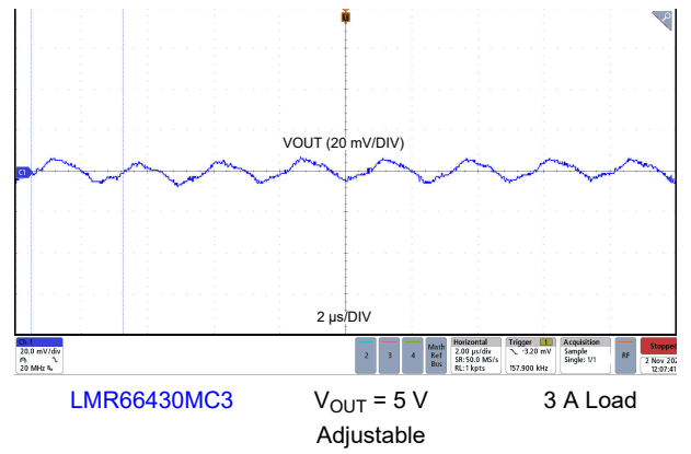
Figure 8-25. Output Voltage Ripple
