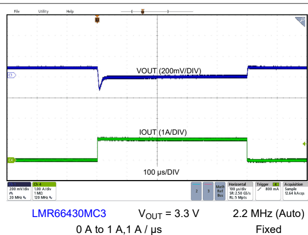
Figure 8-13. Load Transient
