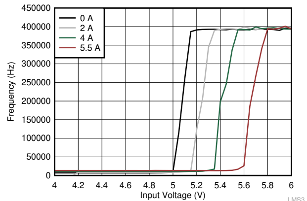
Figure 8-11. Frequency Dropout Characteristics ( V_{OUT} = 5\text{ V} )
