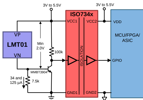
Figure 27. Isolation
