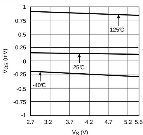
Figure 6. V_{OS} vs Supply Voltage
